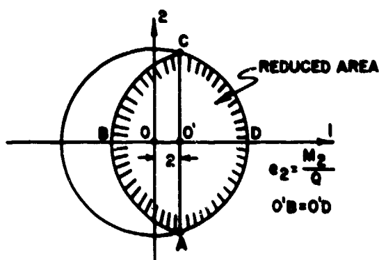
(C) REDUCED AREA-CIRCULAR FOOTING
