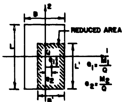
(B) REDUCED AREA-RECTANGULAR FOOTING
