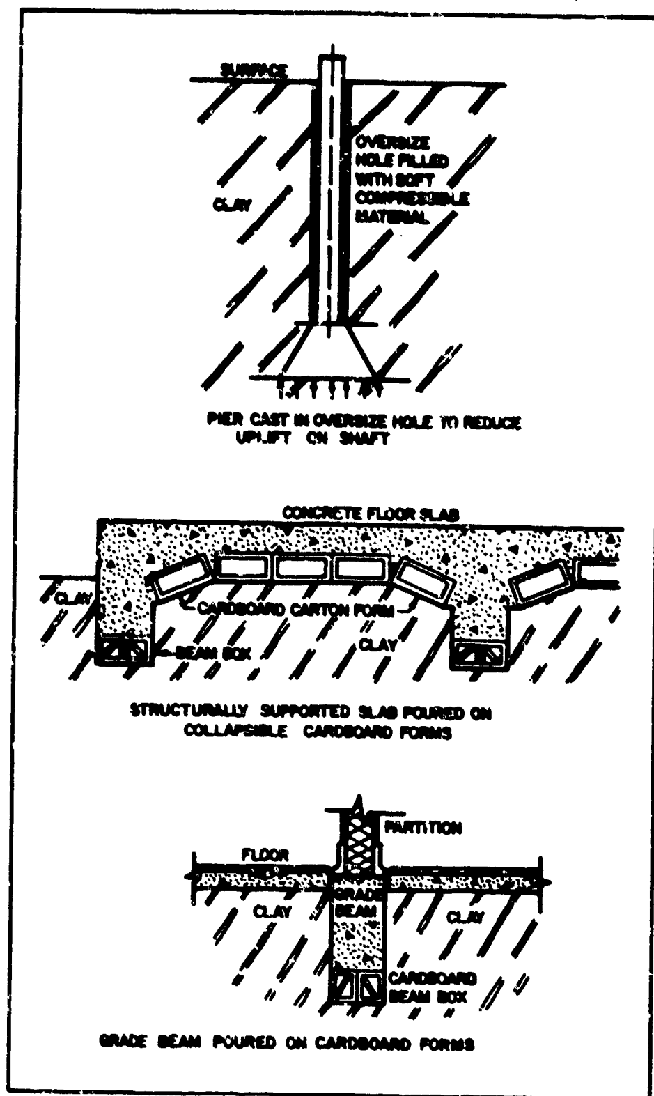
FIGURE 14 Construction Details for Swelling Soils
