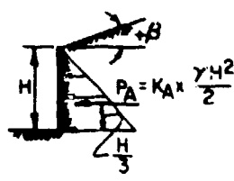
ACTIVE PRESSURE
