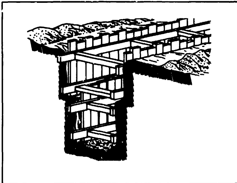
FIGURE 5 Telescopic Shoring
