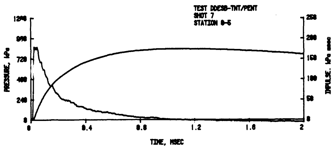
Figure B-10. Pressure and impulse versus time, Station 0-5, TNT.
