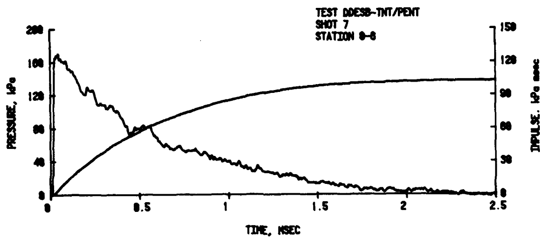
Figure B-14. Pressure and impulse versus time, Station 0-6, TNT.
