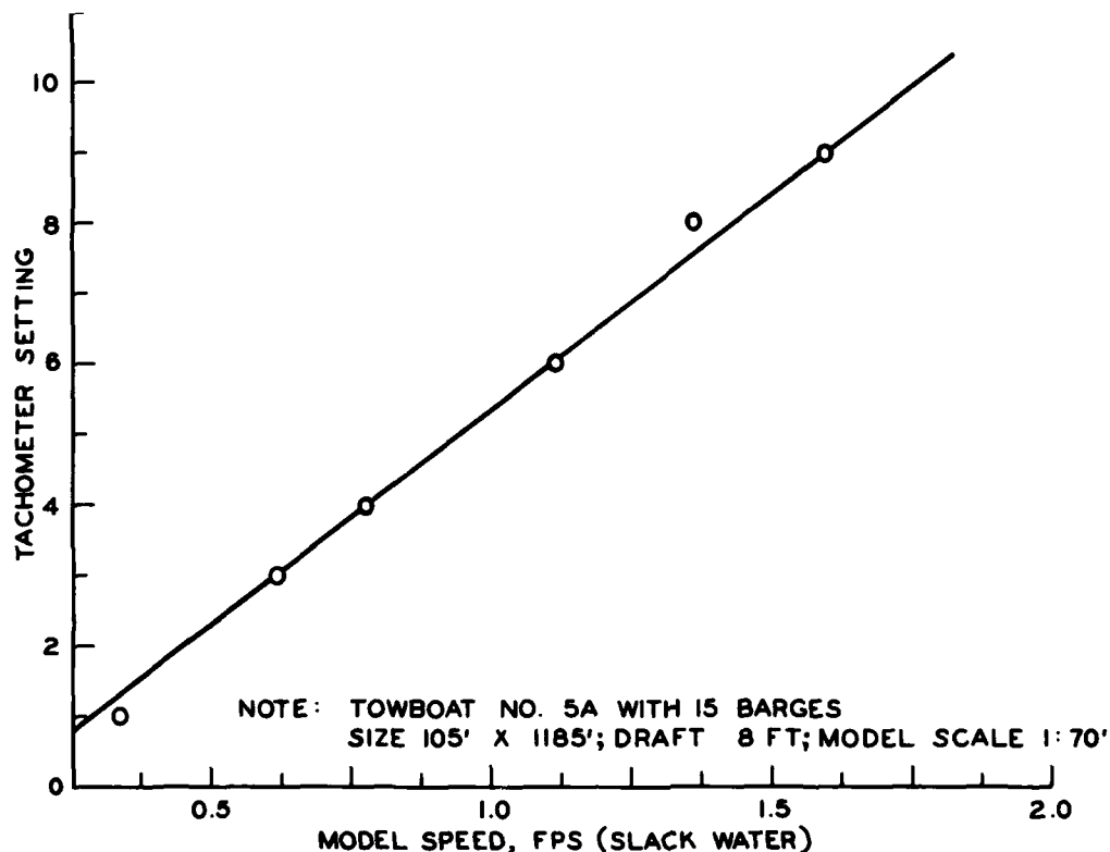
Figure 4. Typical speed calibration curve for model tow
