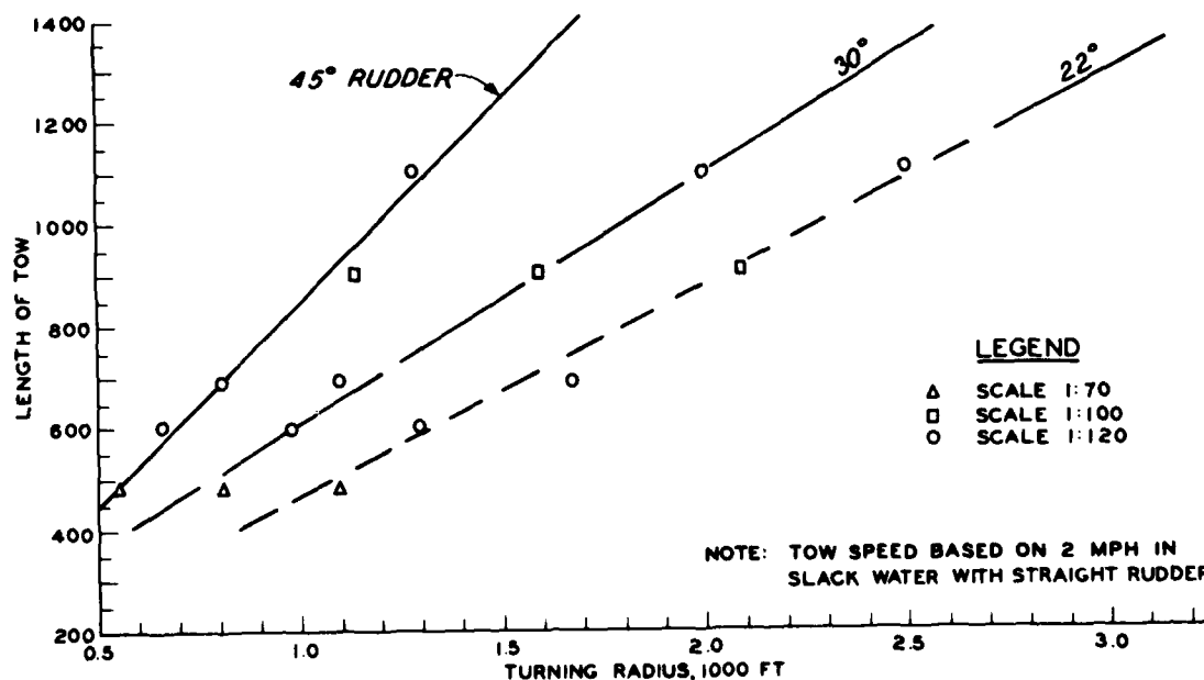
Figure 5. Calibration curves
