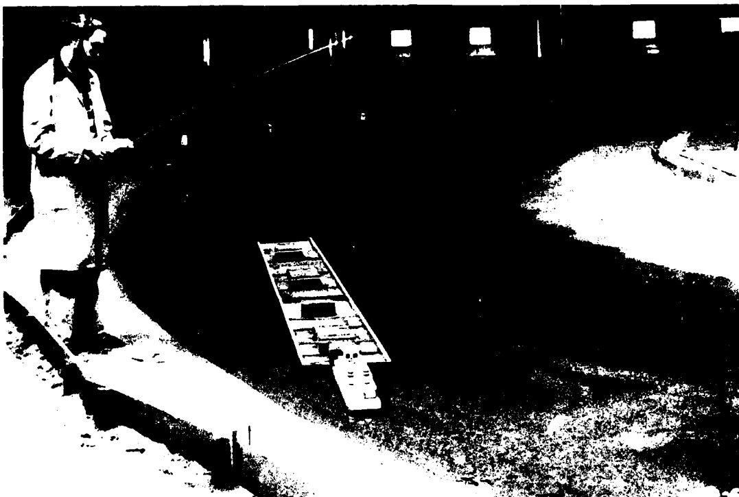
Figure 3. A downbound model towboat and tow negotiating a typical bend
