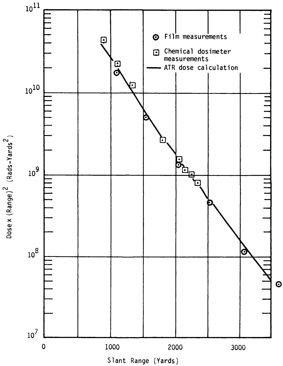
Figure 3-4. Shot Hood Gamma Dose.
