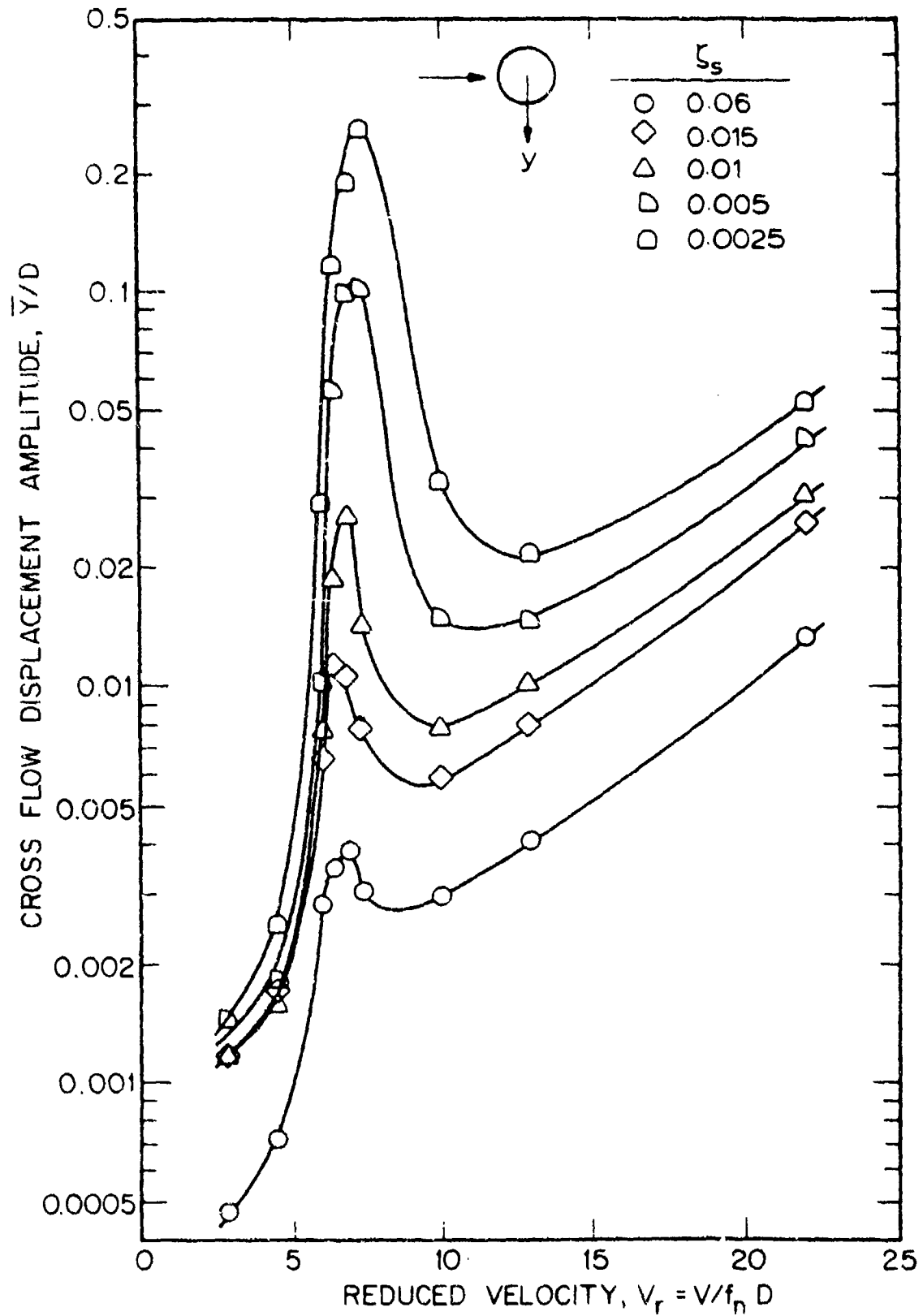
Figure 11. Peak cross flow displacement response \bar{Y}/D (standard deviation of \bar{Y} ) plotted against reduced velocity V_r = V/f_n D for a model circular cylinder in a turbulent boundary layer, from Kwok and Melbourne (31). The structural damping ratio \zeta_s of the rigid pivoted model was varied as shown on the figure. The characteristic flow velocity V was measured at the tip of the cylinder, of aspect ratio L/D = 9 . The figure was provided by Dr. K.C.S. Kwok, University of Sydney, Australia.
