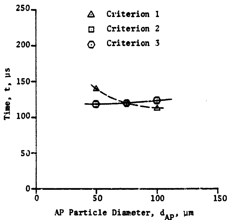
Fig. 14 Predicted Effect of AP Particle Size on Ignition Delays Using Different Ignition Criteria Based Upon the Attainment of: (1) \dot{q}''_{max,critical} ; (2) r_{b,critical} ; and (3) zero axial velocity in the gas phase at a specified location. (Average dP/dt = 120 GPa/s)
