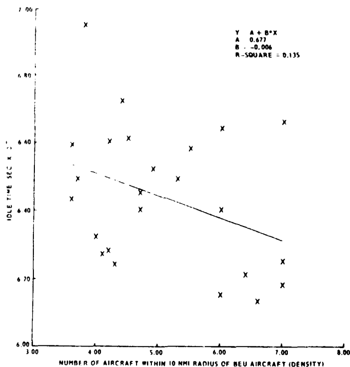
FIGURE 12. DENSITY VERSUS IDLE TIME, LOS ANGELES, JULY 19, 1980
