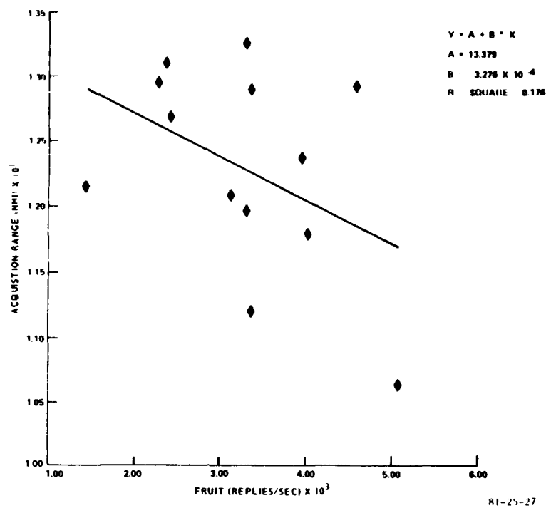
FIGURE 27. ATCRBS ACQUISITION RANGE VERSUS FRUIT — AIRCRAFT N-49 AND N-47, OCTOBER 4, 1980
