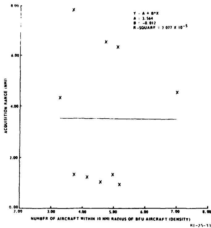
FIGURE 33. ACQUISITION RANGE VERSUS DENSITY — AIRCRAFT N-49 AND N-40, JULY 20, 1980
