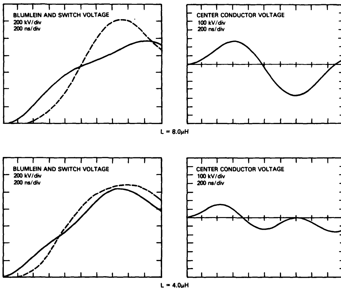
Fig. 10 — Predicted Blumlein voltage monitor (solid line), voltage across the water switch (dotted line), and inner conductor voltages for two different prepulse inductors. Upper: Inductor \sim 8.0\ \mu\text{H} (too large); Lower: Inductor \sim 4.0\ \mu\text{H} (near optimum). The Blumlein voltage waveforms were verified experimentally.
