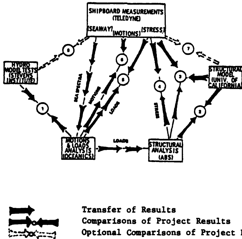
Figure 4-1 SL-7 Data Comparison
