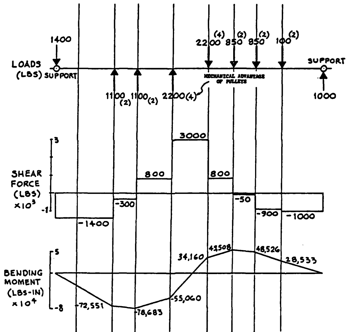
Figure 4-9 Representative Loading Applied to the Steel Structural Model
