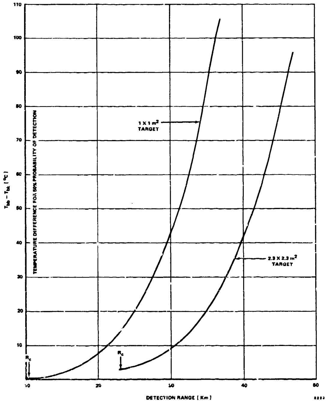
Figure 2 Threat System B T_{bb} = Equivalent Blackbody Temperature of Target T_{bk} = Equivalent Blackbody Temperature of Background
