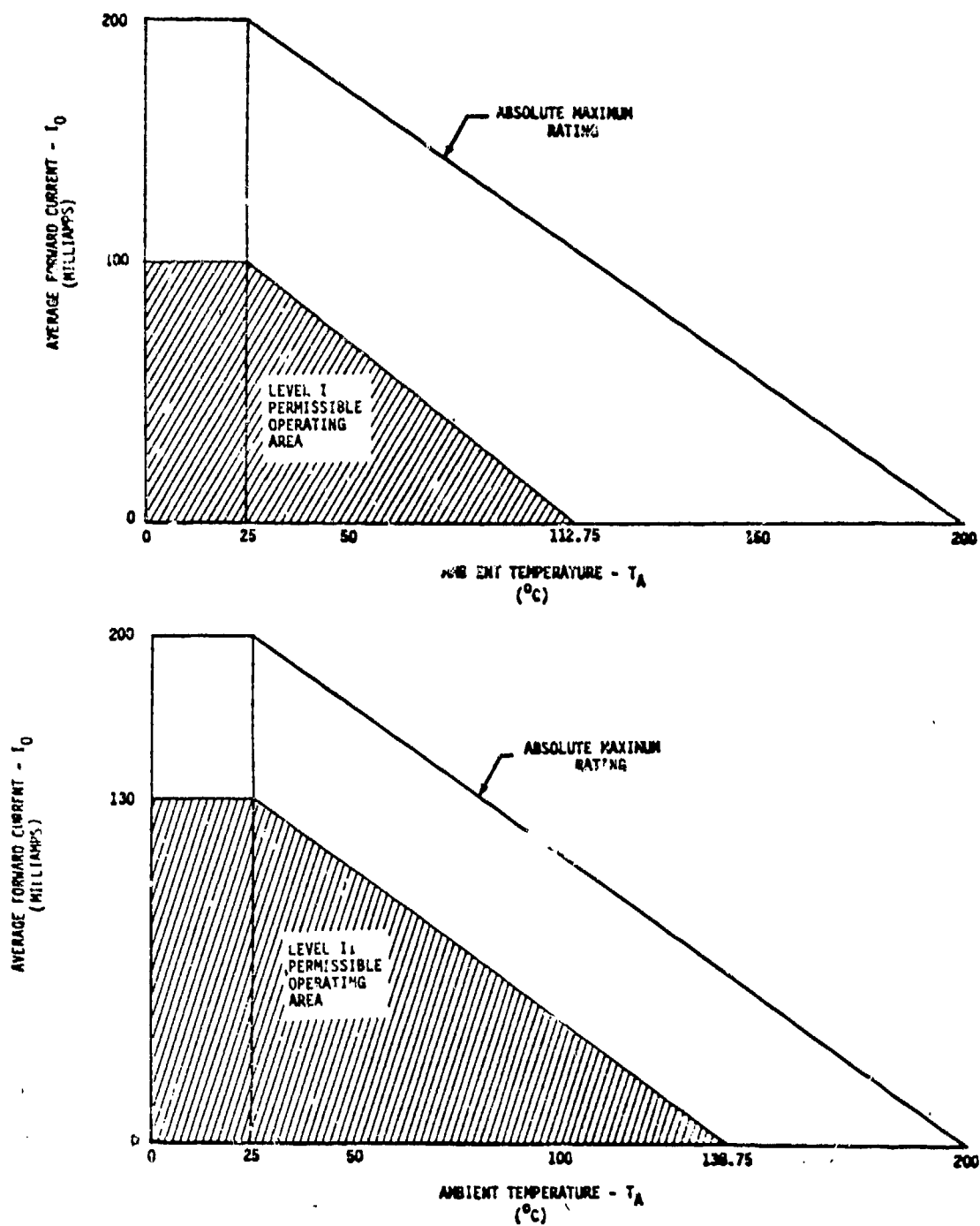
Figure 6-1: Ambient Temperature Derating for Switching Diode Type 1N4148/1N4148-1
