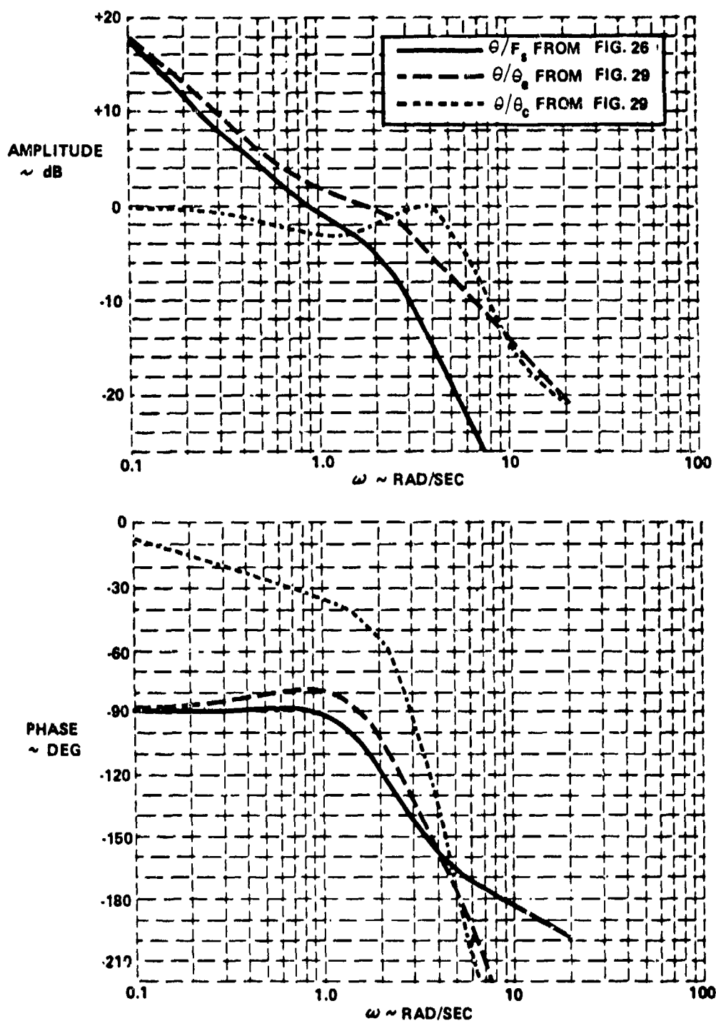
Figure 20. C_1 on-Loop and Closed-Loop Bode Plots for Configuration with Low \omega_{sp}
