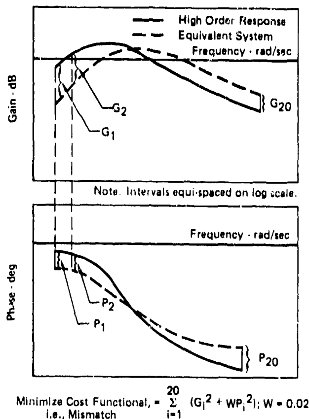
SKETCH OF EQUIVALENT SYSTEM DETERMINATION
