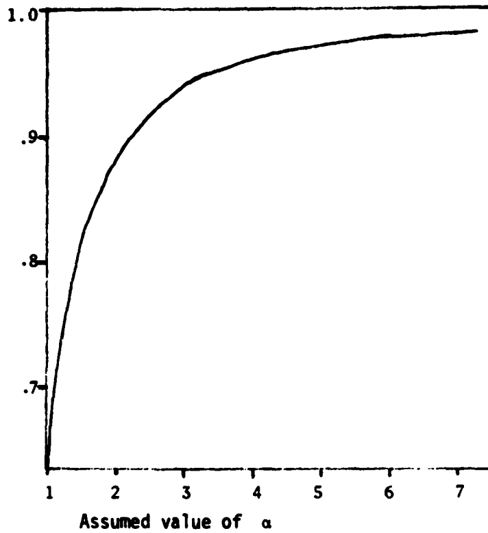
Asymptotic Efficiency of Estimate of Mean of Normal Sample for Assumed Value of \alpha
