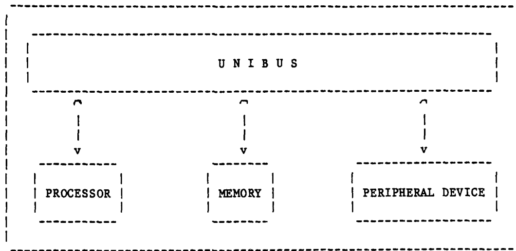
Figure 9. Unibus Configuration
