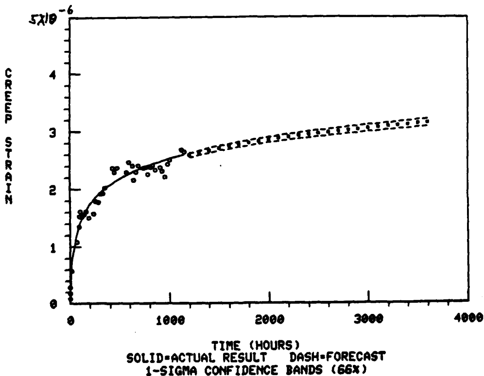
MICROCREEP OF I-400 AT 10 KSI AND 63 CENTIGRADE
