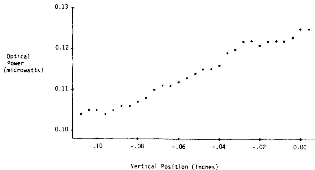
Figure 12. Channel B optical power density.
