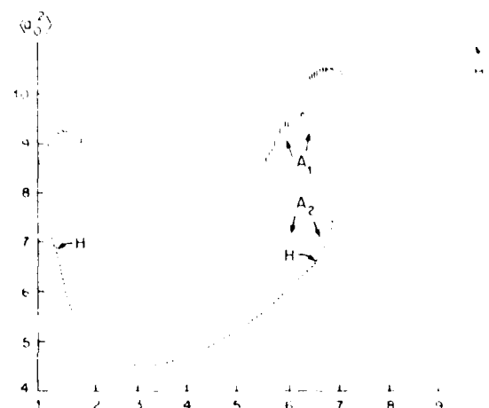
FIG. 4. Hysteresis: the long-time average of a_1 versus \gamma . [|||||]—chaotic behavior, ————limit cycles, ————stable stationary point. H indicates a Hopf bifurcation (A1 and A2 are labels used in the text).
