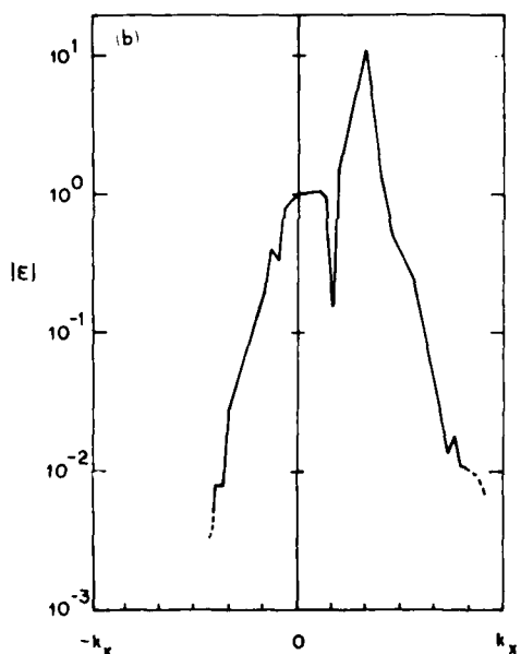
FIG. 4. Electric field amplitude in k space during the one-dimensional simulation at times (a) T = 4.6 \times 10^6 \omega_{pe}^{-1} , showing the enhancement of the pump modes, and (b) T = 6.7 \times 10^6 \omega_{pe}^{-1} , showing many of the same features seen in Fig. 3(b). The amplitudes of 60 wave modes centered at zero are shown. The largest wavenumber k_x is 0.025 \lambda_e^{-1} .
