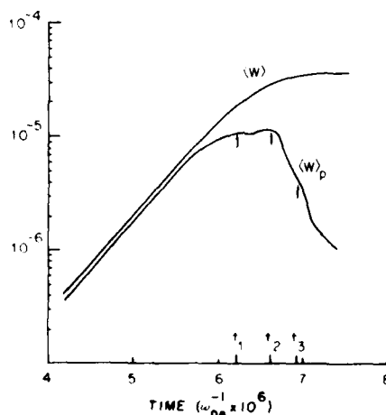
FIG. 1. Energy density in the pump resonant modes, \langle W \rangle_p , and total energy density \langle W \rangle during the two-dimensional simulation of a type III burst at 0.5 a.u.
