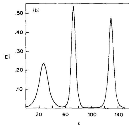
FIG. 6. Electric field amplitude in real space during the one-dimensional simulation at times (a) T = 6.9 \times 10^6 \omega_{pe}^{-1} and (b) T = 9.9 \times 10^6 \omega_{pe}^{-1} , spanning several beam growth time scales. Labels are in the dimensionless units [E] , [x] . In dimensional units, x = 100 corresponds to 4500 \lambda_e .
