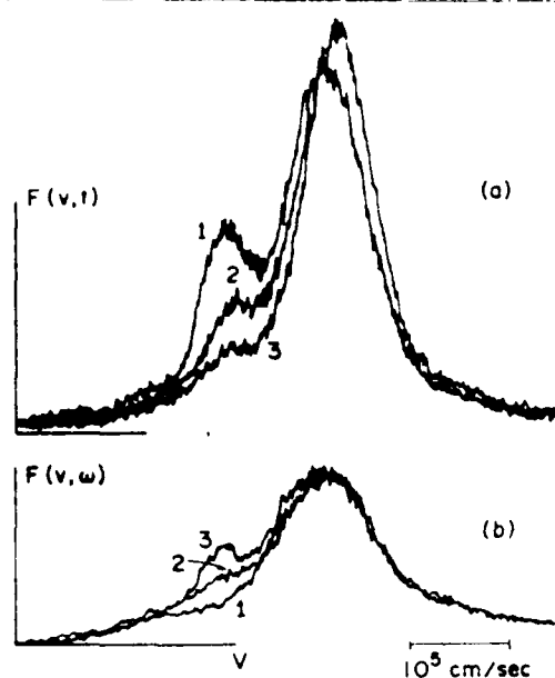
FIG. 3. Evolution of the ion beam in time. Vertical: F(v, t) , ion distribution function, linear scale, and arbitrary units. Horizontal: ion velocity v , linear scale indicated. Position is r = 12 \text{ mm} . (a) Phase locked with reference from EICW oscillation and (b) radio signal. (1) and (3), radio tuned to \omega , excitation on and off, respectively; (2), radio detuned ( \omega' ), excitation on.
