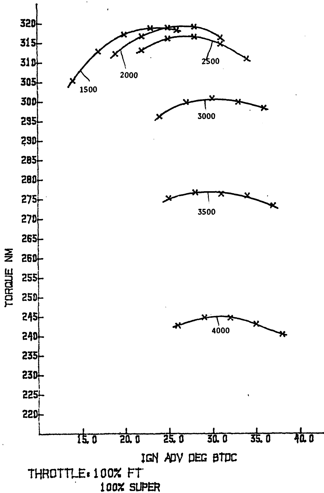
FIG 8 - TORQUE vs IGNITION ADV (MBT)
