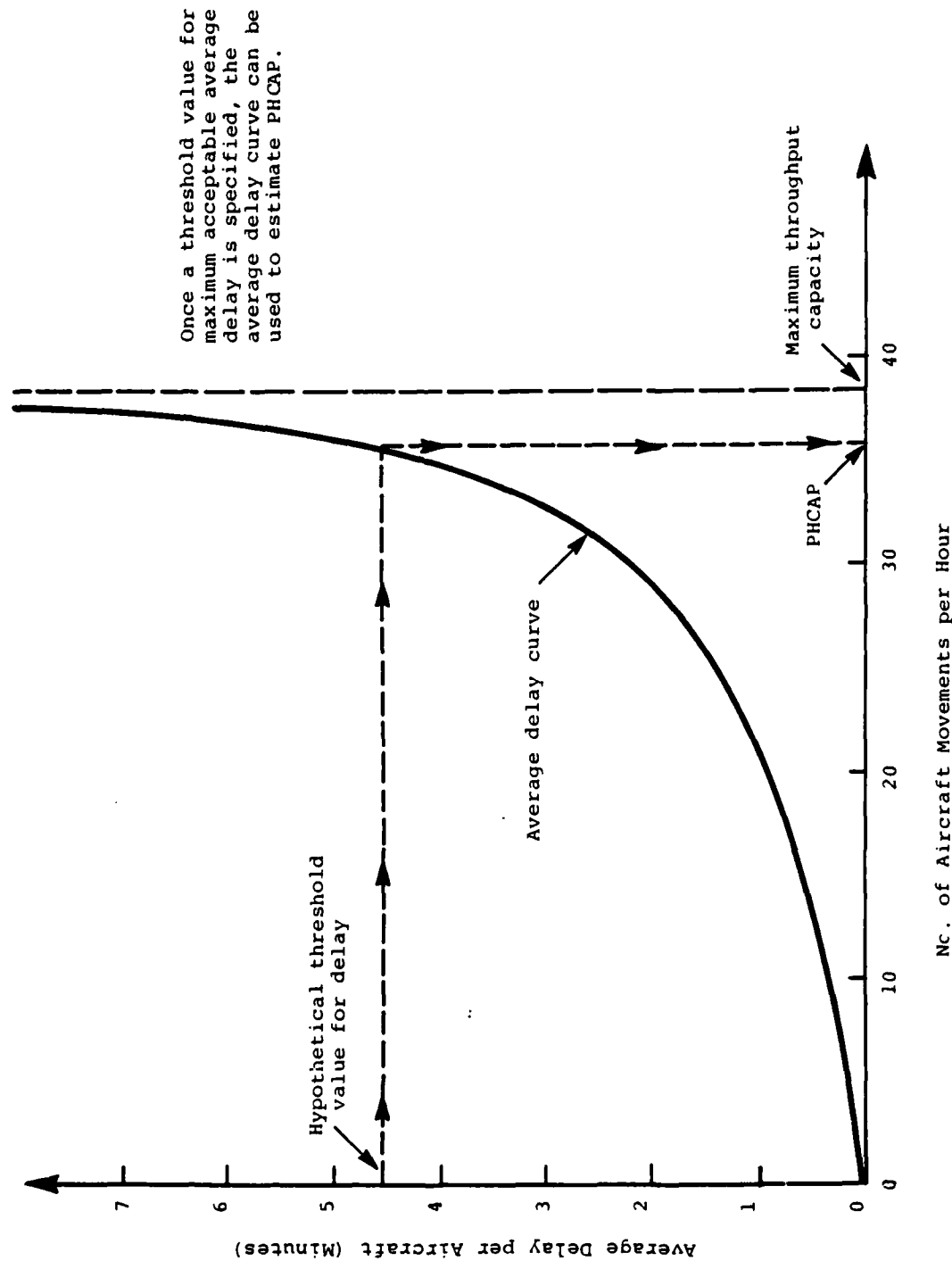
FIGURE C-1. AVERAGE DELAY VS. HOURLY TRAFFIC MOVEMENT
