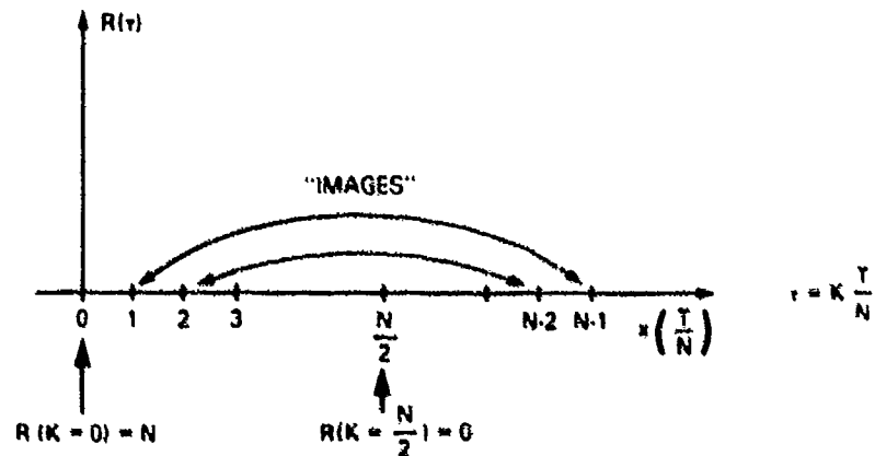
Fig. 4 - Image structure of the autocorrelation function of an even-length Barker code
