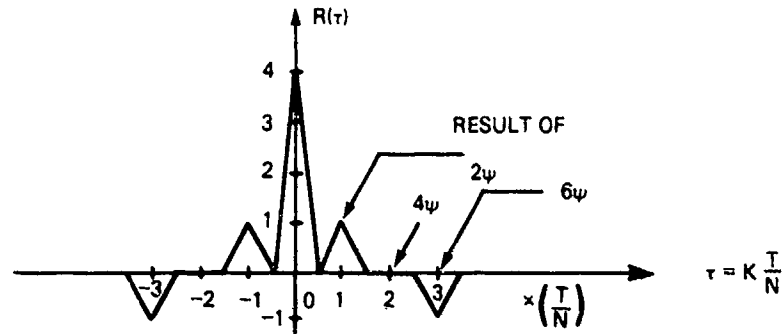
Fig. 3 - Autocorrelation function of Barker code 4A
