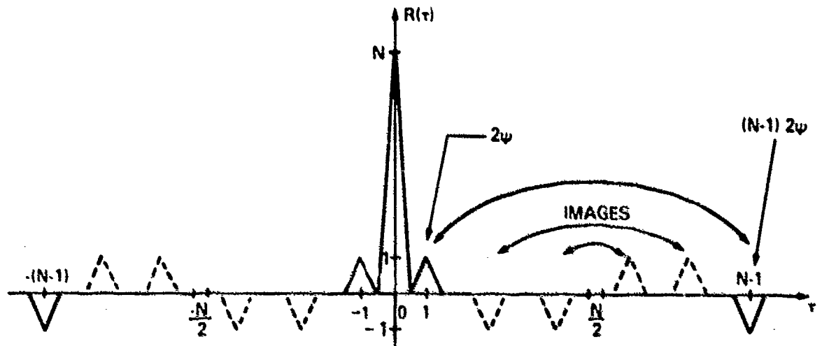
Fig. 6 - Autocorrelation function of even-length Barker codes (generally)
