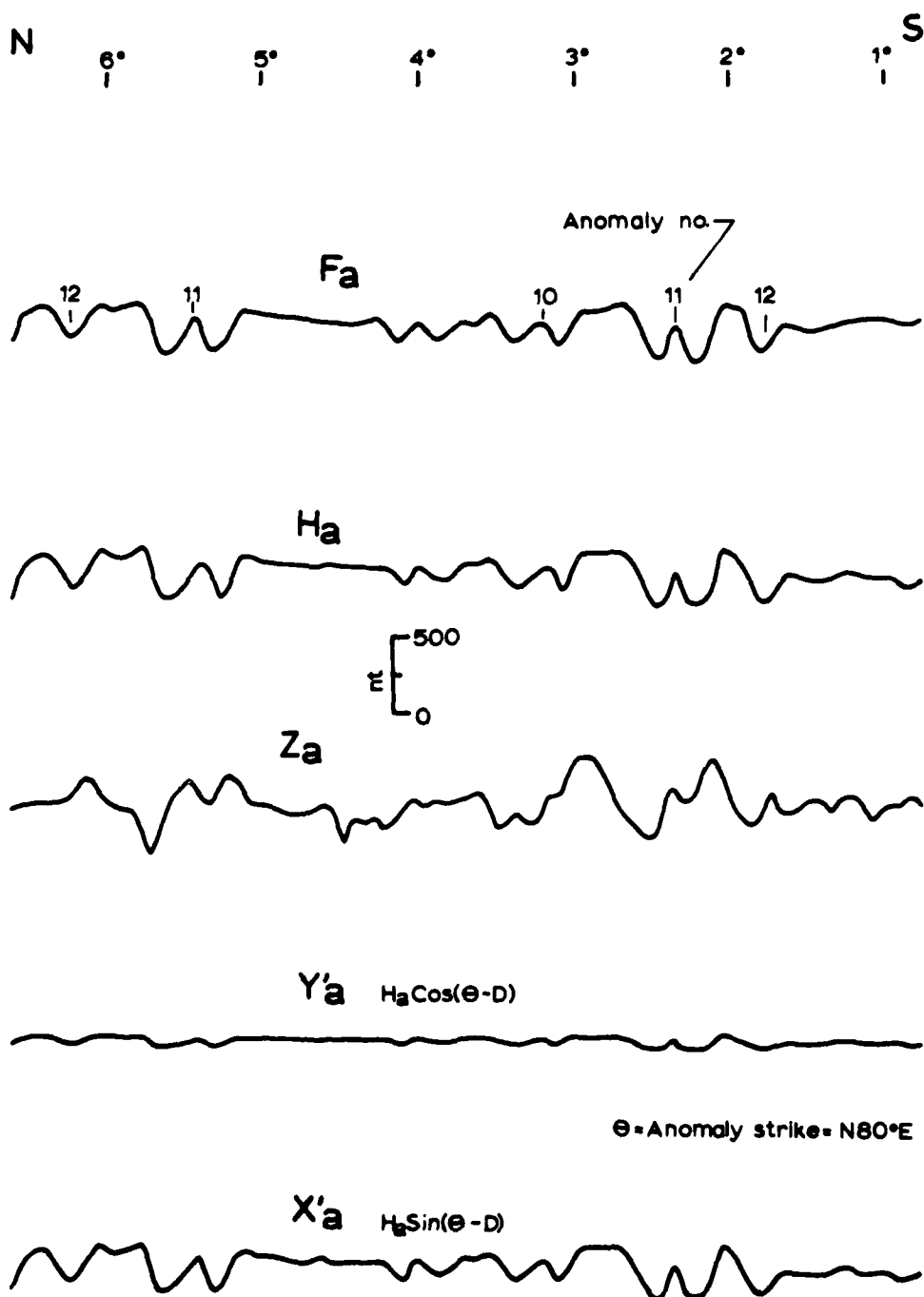
Figure 1. Example of magnetic component data over two-dimensional sea-floor spreading anomalies (from Sracey, 1981B).
