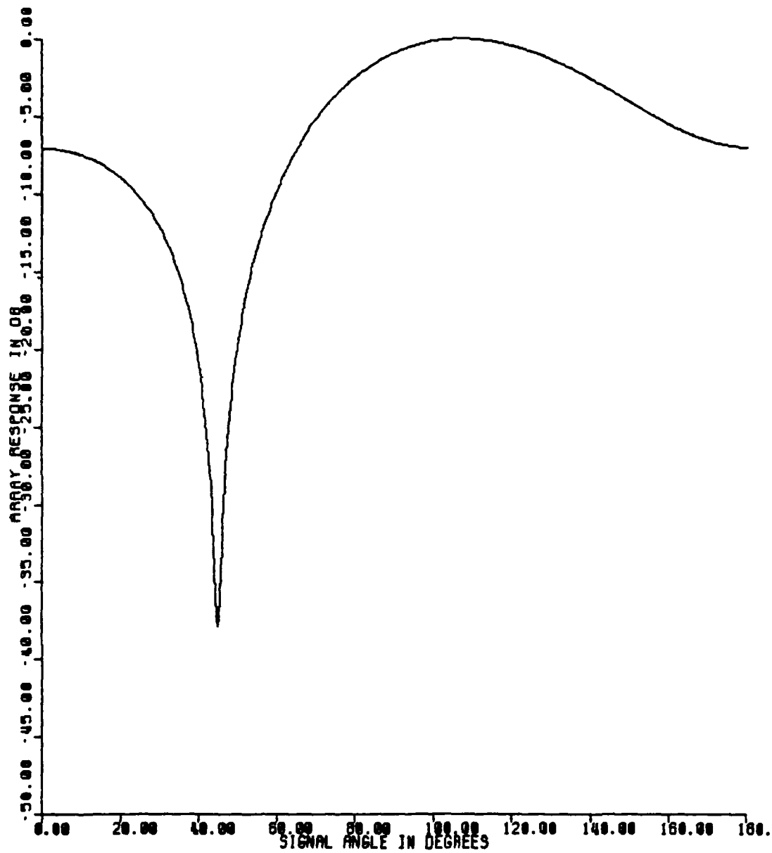
FIGURE 2-24: Spatial Response for 20° Uniform Extended Source at 45° d/\lambda = .5 , m=1 , K=1 , INR=40 dB
