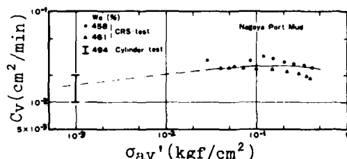
Fig.23 \log C_v vs \log \sigma_{av}' relation ( Nagoya Port muds )
