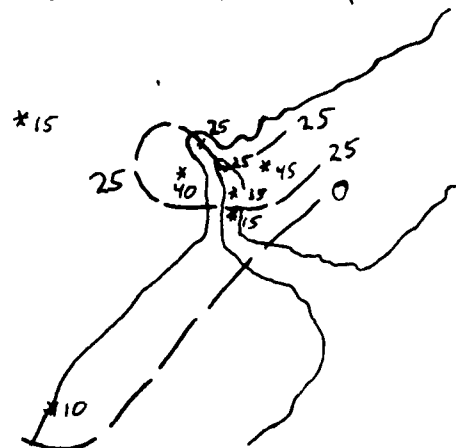
minimum T Figure 2-11. Minimum shelf water temperature and depth of the cold pool near Baltimore, Wilmington, and Hudson Canyons. Limits of cold pool were taken at 35% and 11%. thickness (m)
