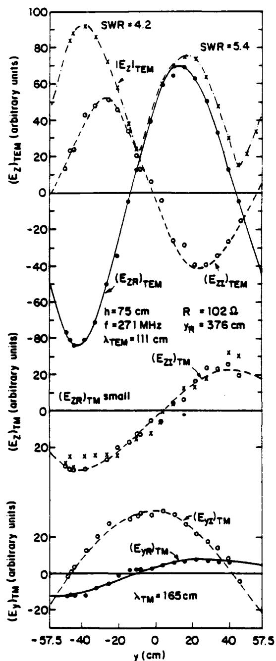
Figure 8. TEM and TM components of the electric field in the parallel-plate region. (E_z)_{\text{TEM}} = E_z(z/h=0.5) (E_z)_{\text{TM}} = E_z(z/h=0) - E_z(z/h=0.5) = E_z(z/h=0.5) - E_z(z/h=1) [denoted respectively by o and x in graph for (E_z)_{\text{TM}} ]. E_z = |E_z| \exp(i\theta_z) = E_{zR} + iE_{zI} ; \theta_z = 0 at x = y = z = 0 .
