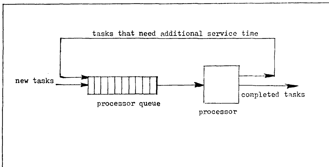
Figure 11 Round-Robin Model
