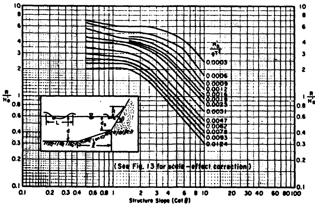
Figure 6. Relative runup for smooth slopes on a 1 on 10 bottom; L/L \geq 0.5 ; d_s/H'_0 = 1.5 (from Stoa, 1978).
