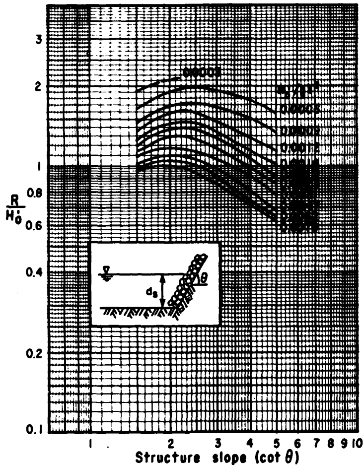
Figure 4. Relative runup for riprap slopes; d_s/H'_0 = 8.0 ; H'_0/K_r = 2.8 . Use this figure also for d_s/H'_0 > 8.0 (from Stoa, 1979).
