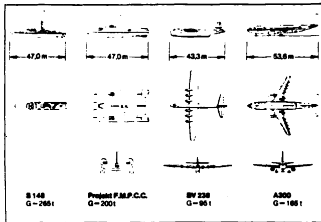
Fig. 21: Size comparison of a Class 148 fast attack craft, an FMPCC, a BV-238 flying boat and an A 300 Airbus.
