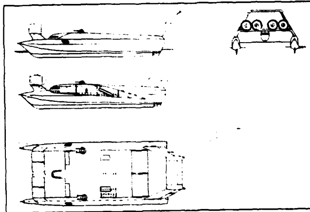
Fig. 23: Project of an FMPC according to the PAR WIG System with an operational displacement of 511 tons.
