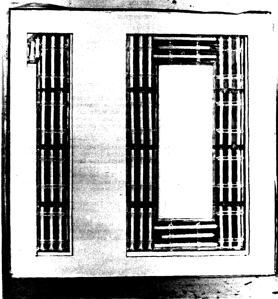
FIGURE 1. Runway Distance Marker With Front Face Removed to Show Tritium-Filled Phosphor Coated Tubes
