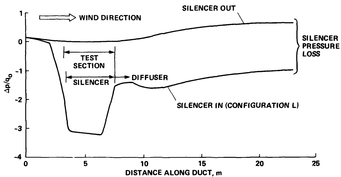
Figure 28.— Typical static pressure change along the duct normalized by free-stream dynamic pressure, with and without silencer installed: U_0 \approx 24 m/sec.
