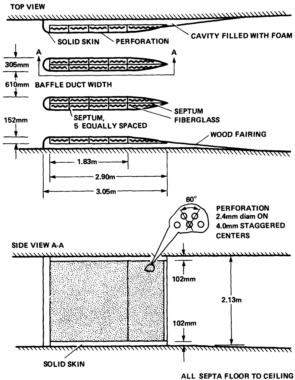
(c) Dimensions.
