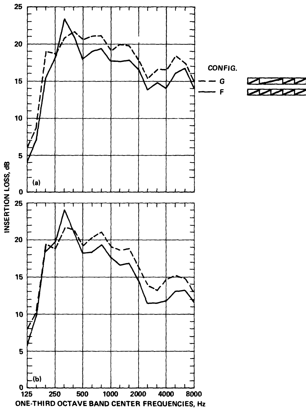
Figure 13.— Comparison of two triangular cavity geometries; both configurations had cavity linings. (a) U = 0 , inlet simulation. (b) U \approx 19 m/sec, inlet simulation.
