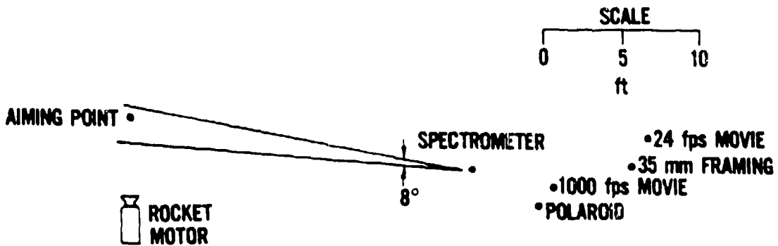
FIGURE 3. TEST SET-UP
