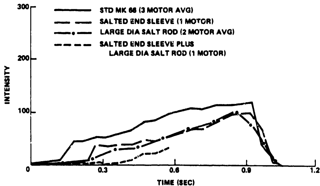
FIGURE 7. HUMAN EYE ADJUSTED EMISSIONS
