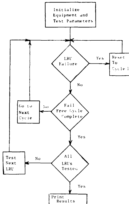
FIGURE 7 COMPUTER FLOW DIAGRAM-PVT
