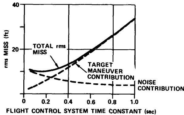
Figure 3. Flight Control System Time Constant Influences System Performance
