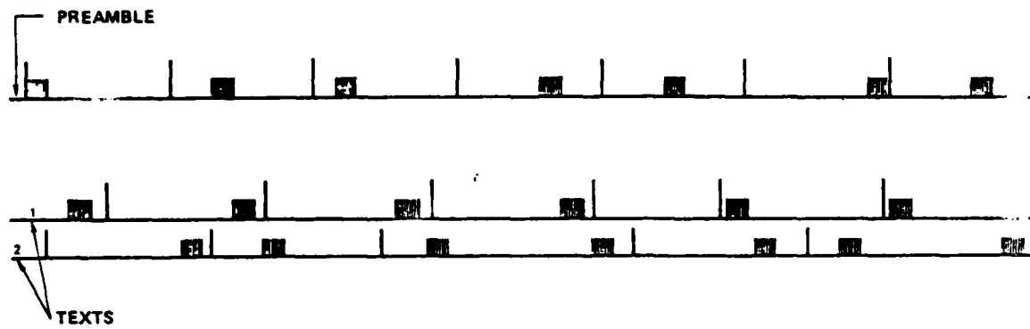
Fig.6 Jamming of the preamble by the text
