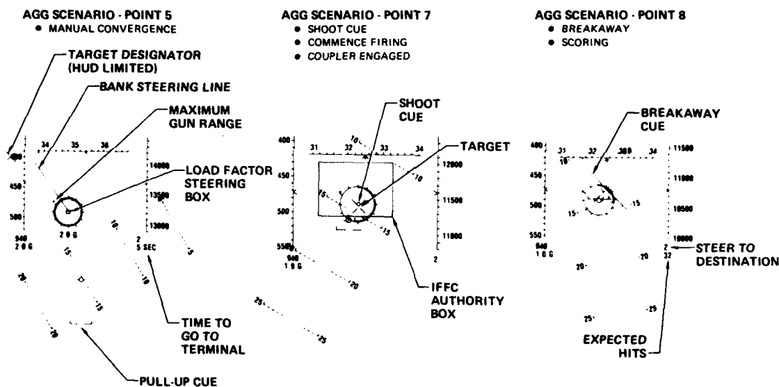
Figure 14. HUD Display During IFFC Air-to-Ground Gunnery Scenario
