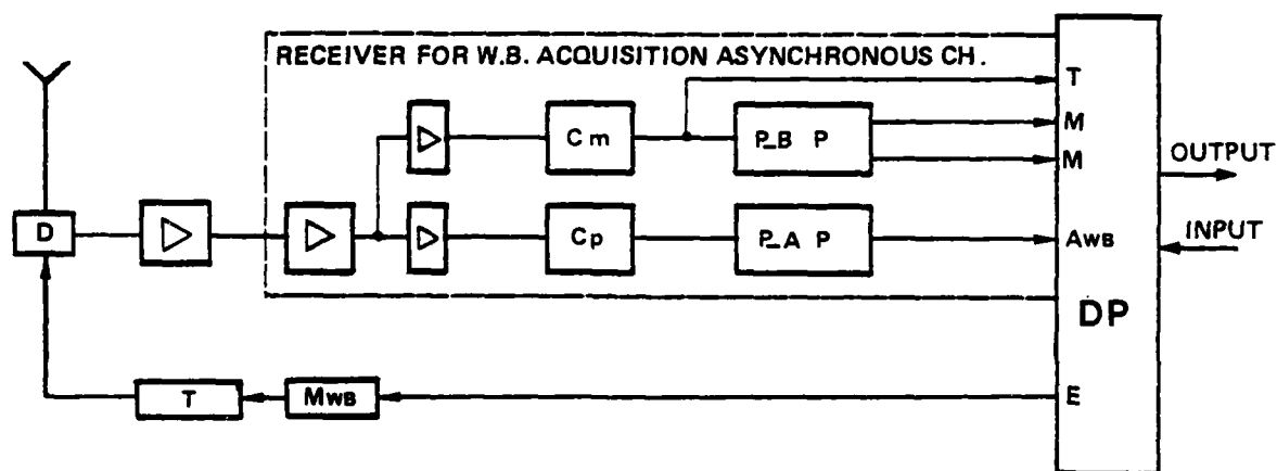
Fig.10 Terminal B6
