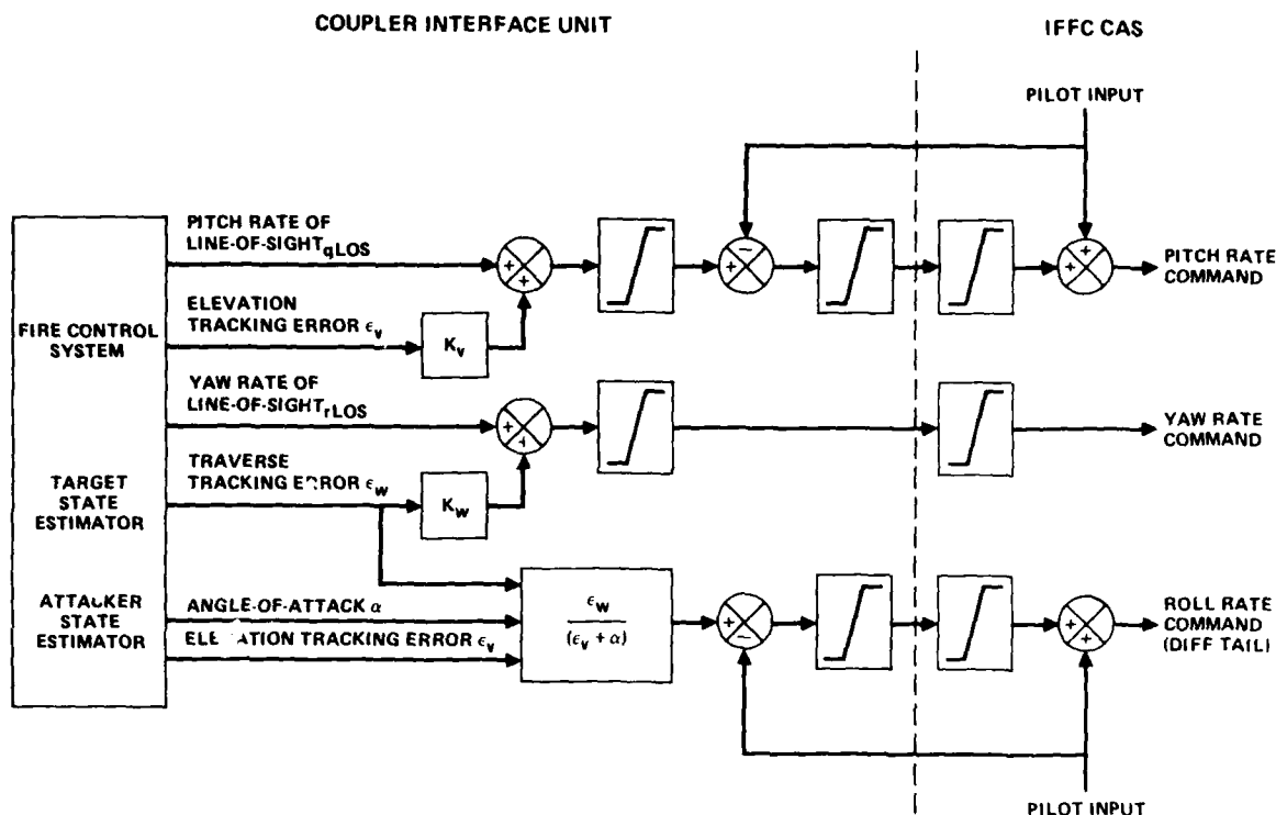
Figure 8. Air-to-Air Gunner Coupler Control Laws
