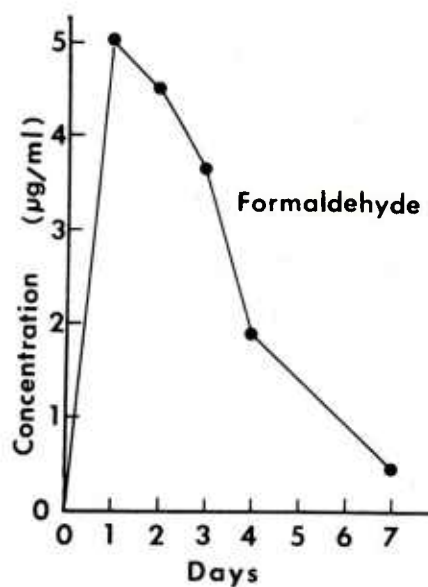
Figure 5. Kinetics of formaldehyde formation.
