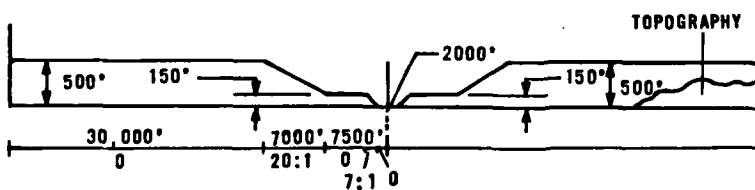
ELEVATION AT RIGHT ANGLES TO RUNWAY
