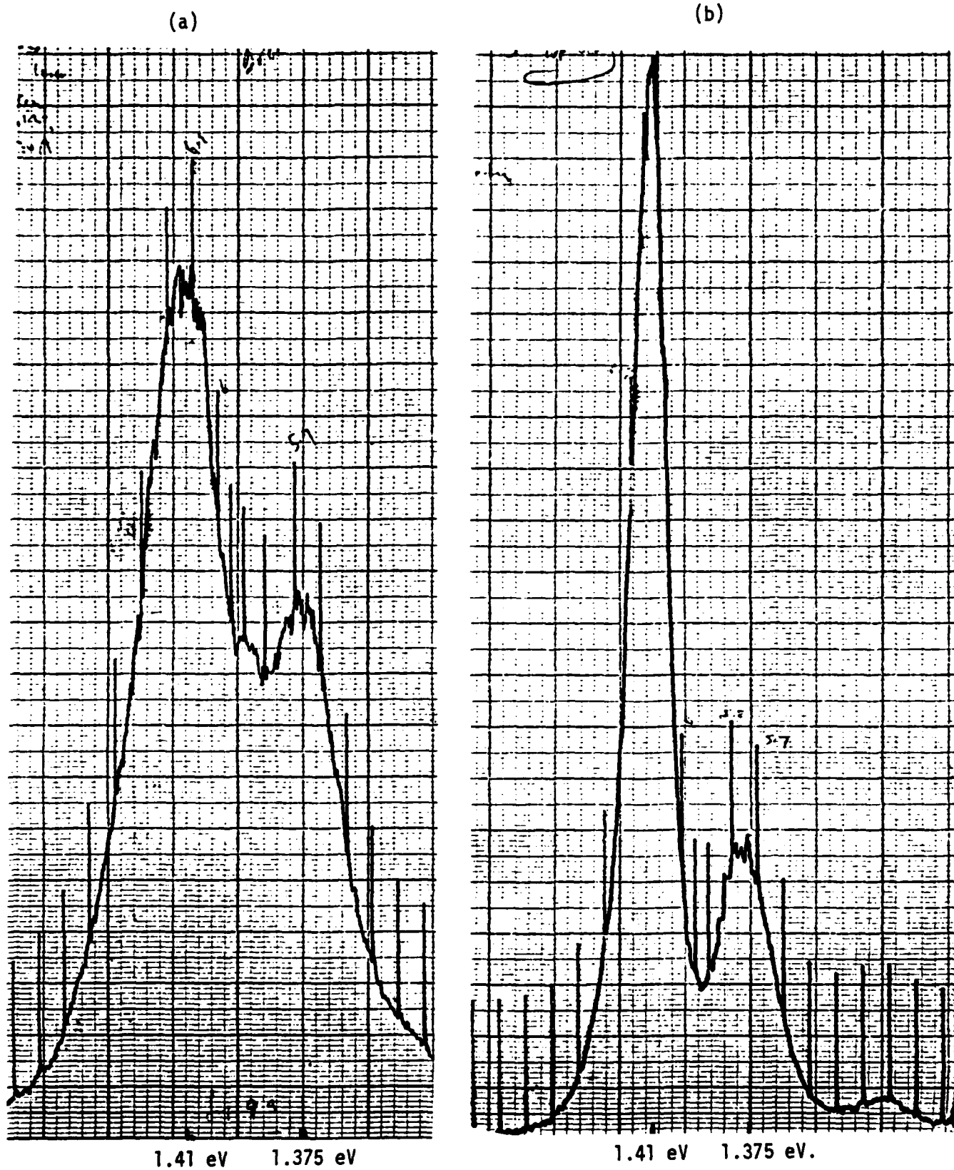
Fig. 9 77°K photoluminescence spectra of poly InP grown by solute diffusion in the (a) upper tray and (b) lower tray.
