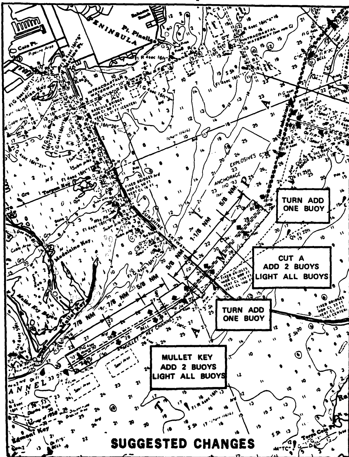
Figure 2-8. Recommended Buoy Configurations for Mullet Key and Cut A Channels, Tampa Bay (Chart 11414, March 28, 1981, With Additions)
