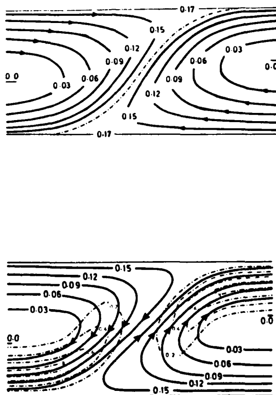
Figure 8. Results of Moncrieff's analytical (a) and numerical (b) model for R = \frac{1}{2} . Chain line in (a) represents the interface between the updraft and downdraft. In (b) the nondimensional temperature excess is shown as a chain line (From Moncrieff, 1978.)
