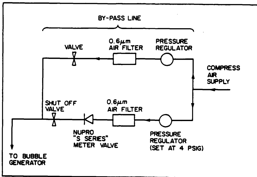
Fig. 4.1. Diagram of the air bubble injection system.
