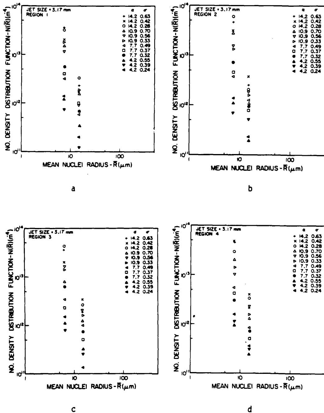
Fig. 5.40. Plots of the nuclei distributions for the 3.17mm jet: (a) Region 1, (b) Region 2, (c) Region 3, and (d) Region 4.
