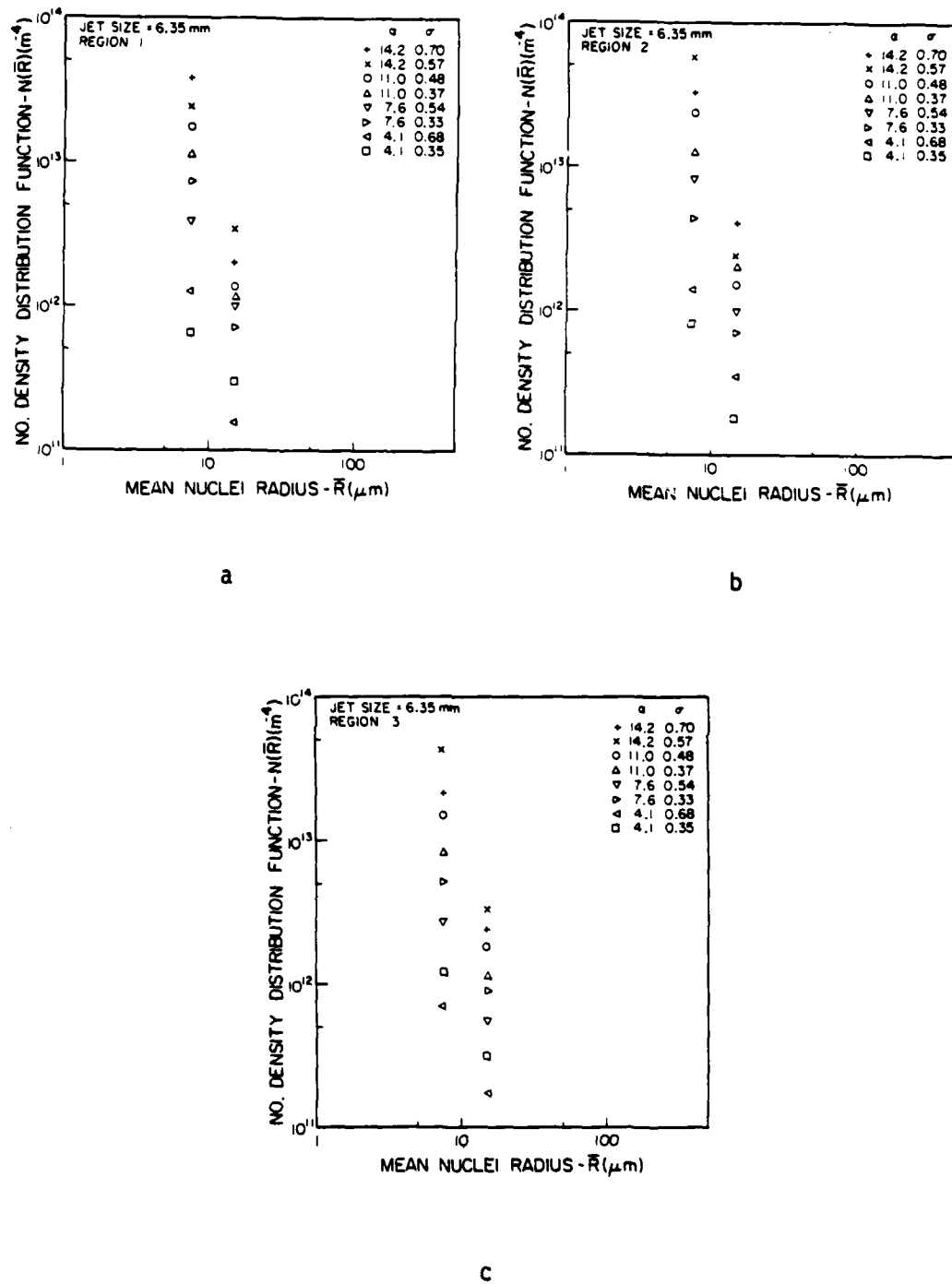
Fig. 5.42. Plots of the nuclei distributions for the 6.35 mm jet: (a) Region 1, (b) Region 2, (c) Region 3.
