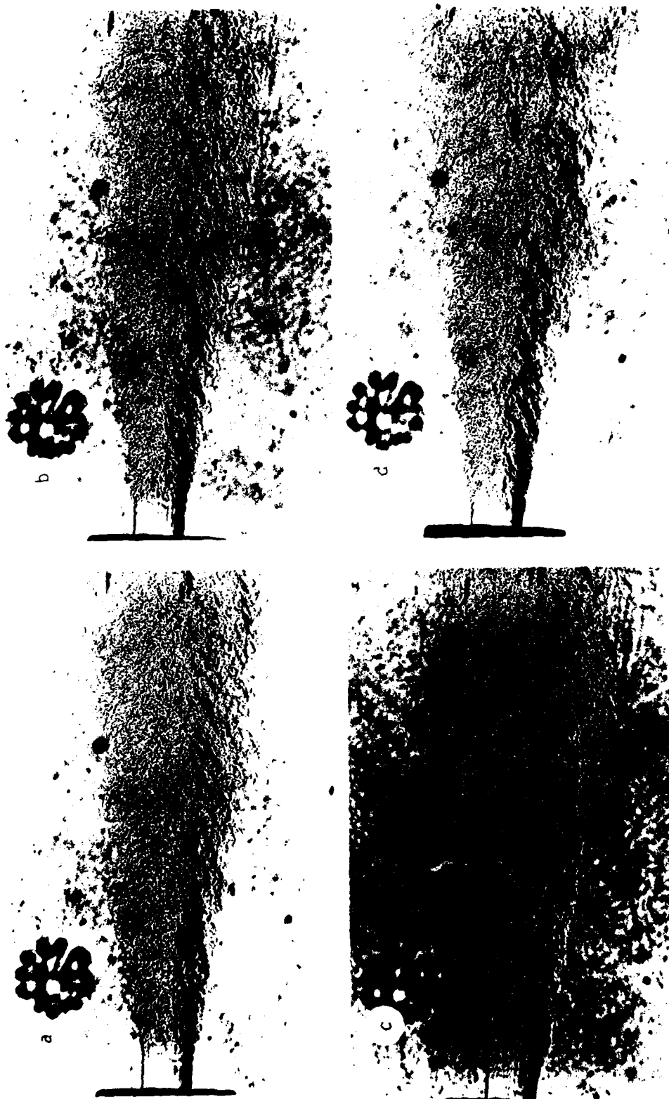
Fig. 5.35. Schlieren photographs of the non-cavitating 3.17\text{mm} jet taken with the knife edge parallel to the flow direction: (a) Re_D = 1.50 \times 10^3 , (b) Re_D = 3.57 \times 10^3 , (c) Re_D = 4.48 \times 10^3 , (d) Re_D = 7.67 \times 10^3 .
