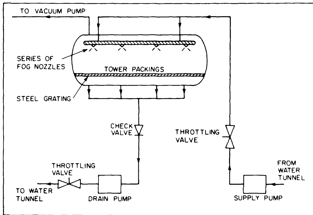
Fig. 2.2(a). Schematic diagram of the dearator system.
