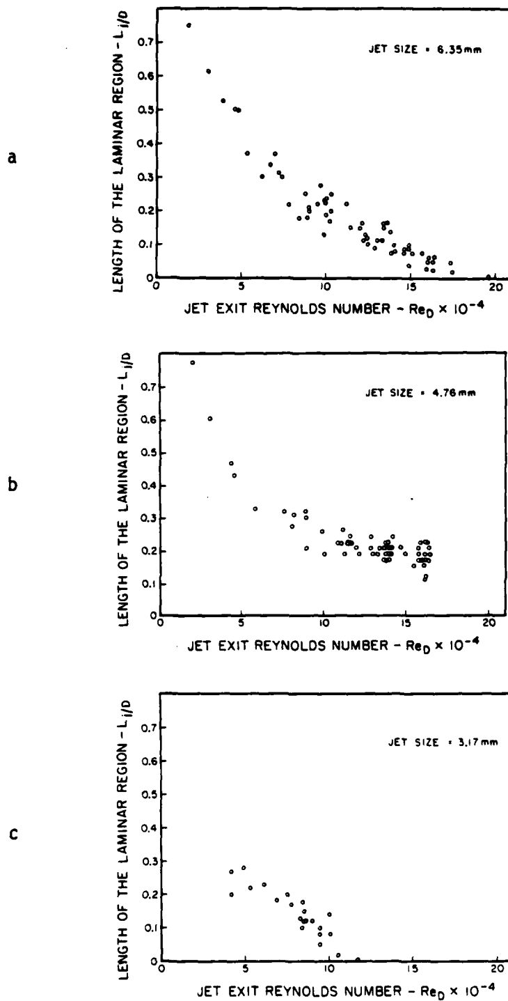
Fig. 5.37. Graphs of L_j/D vs Re_D for the (a) 6.35mm jet, (b) 4.76mm jet, and (c) 3.17mm jet.
