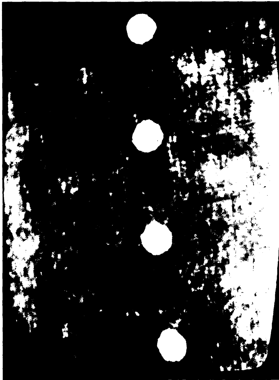
Fig. 3.3. Photograph of the reconstructed image of a string of injected bubbles in the potential core of the jet, near the nozzle exit. The bubbles are 1.3 \text{ mm} in diameter.
