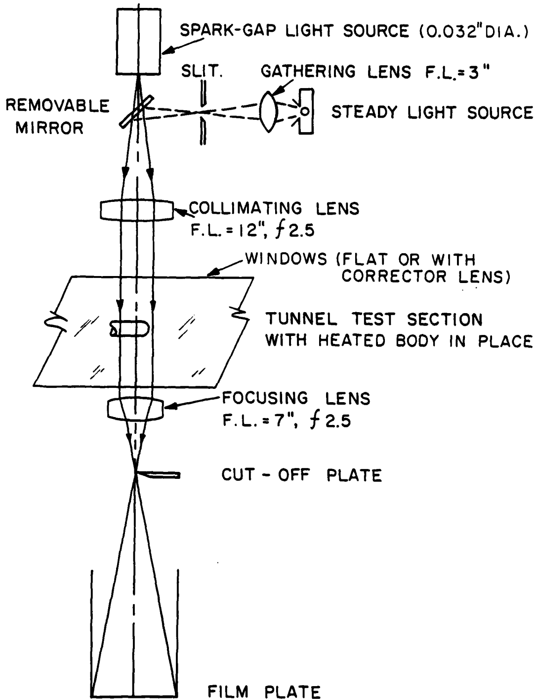
Fig. 2.8. Schematic drawing of the schlieren system (Gates 1977).
