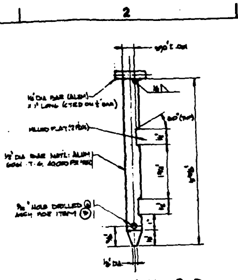
DETAIL 2-D SHEAR PIN (10 REQ'D, INCLUDING SPARES) SCALE: FULL SIZE
