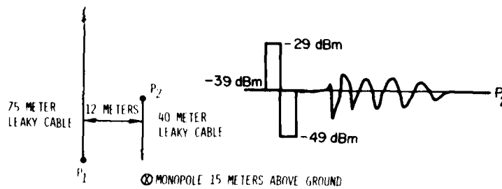
Figure 9a. Power Received From 40 m Cable From a Monopole 15 m Above Ground
