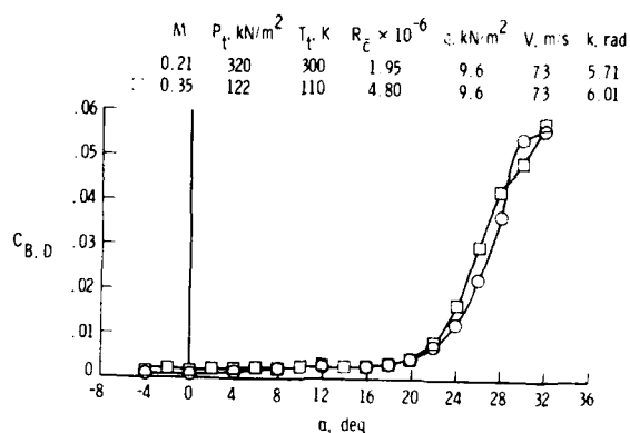
Figure 13.- Comparison of ambient and cryogenic buffet data for the delta-wing model.
