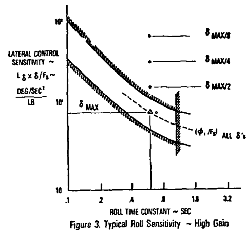
Figure 3. Typical Roll Sensitivity ~ High Gain
