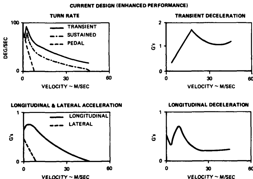
Fig. 4 Maximum Maneuver Capability
