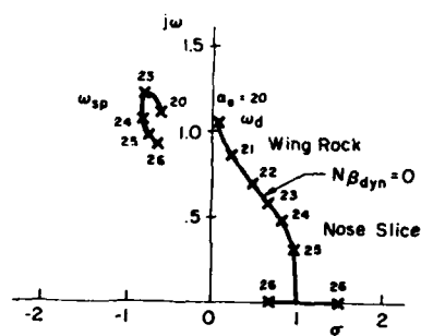
Lateral/Longitudinal Root Migration With \alpha
