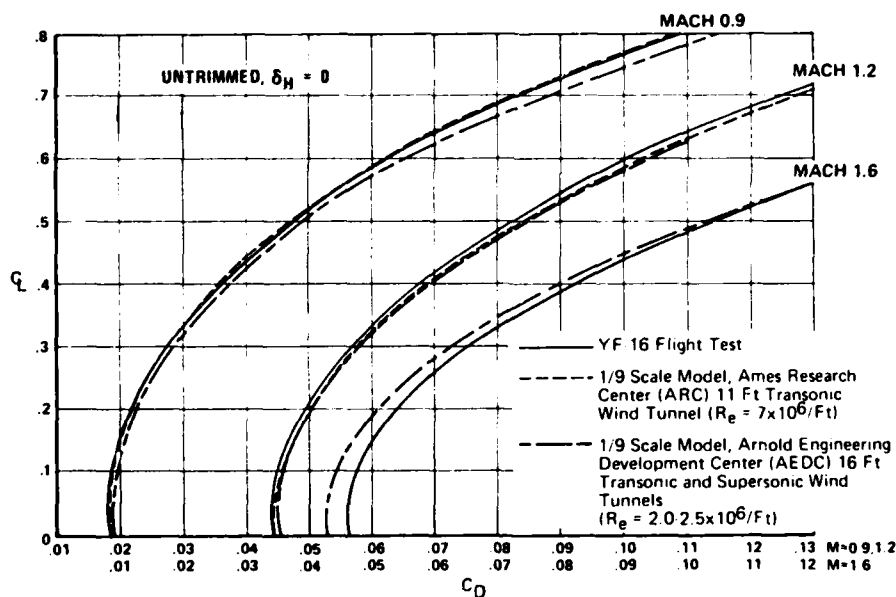
Comparison of Flight Test With Wind Tunnel Drag Polars for YF-16
