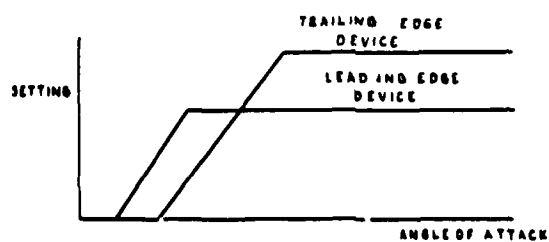
FIG. 4 TYPICAL MANOEUVRE DEVICE SCHEDULES FOR OPTIMUM LIFT/DRAG RATIO
