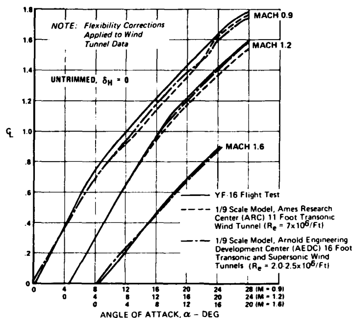
Comparison of Flight Test With Wind Tunnel Lift Curves for YF-16
