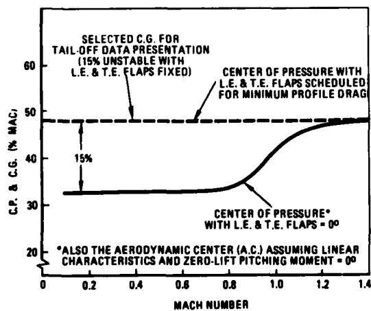
FIGURE 9. C.G. AND TAIL-OFF C.P. POSITION AT LOW \alpha ( 0^\circ - 10^\circ )
