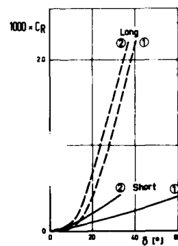
HINGE MOMENTS COMPARISON BETWEEN LONG AND SHORT FLAP CONFIGURATION
