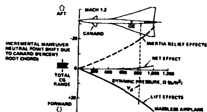
Effect of Aeroelasticity on Canard Contribution to Longitudinal Stability
