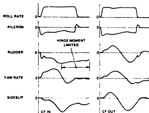
Fig.18. MANOEUVRING LIMITATIONS
