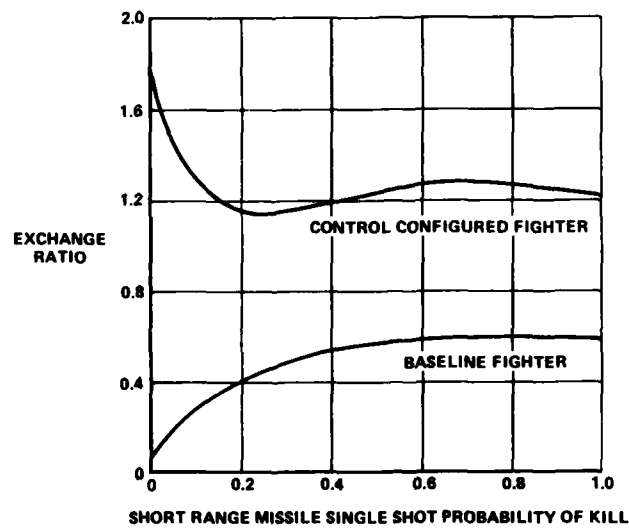
Figure 10. Control Configured Fighter Advantage at All Missile Lethalities One Versus Two Manned Simulation
