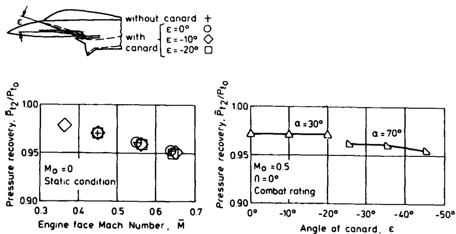
Effect of canard on pressure recovery
