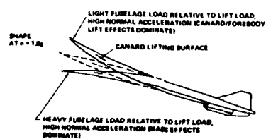
Aeroelastic Effects of Canard in Maneuvering Flight
