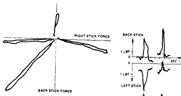
Fig.11. OPEN LOOP TEST CHARACTERISTICS OF FORCE STICK (RAE TEST RIG)
