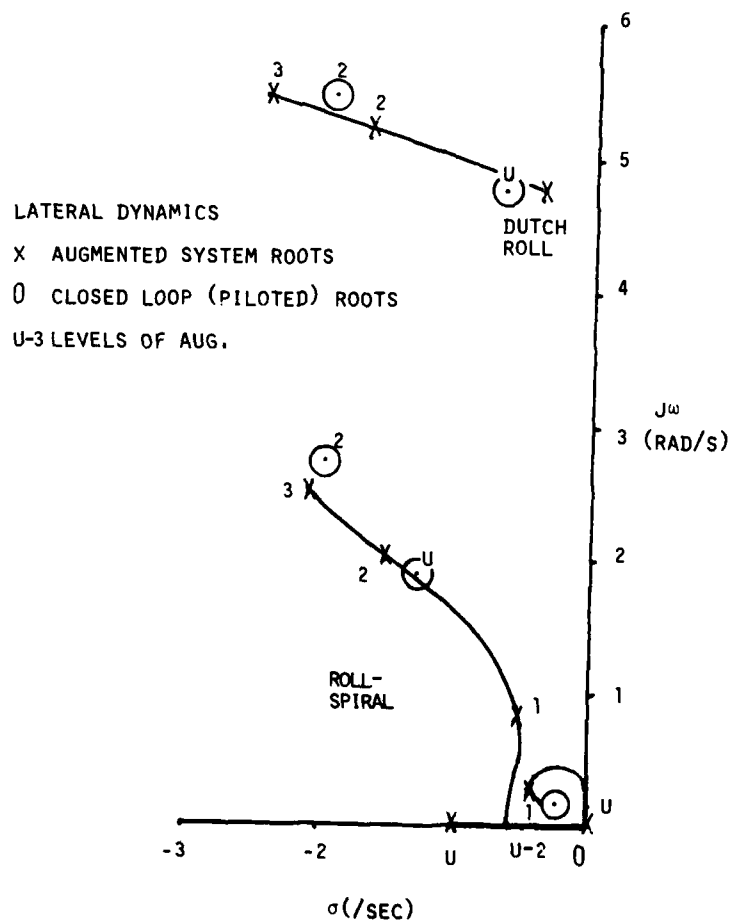
Fig. 7 Lateral-Directional Dynamics
