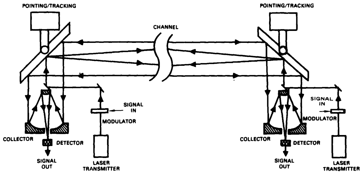
Figure 1. Conventional optical communications system.
