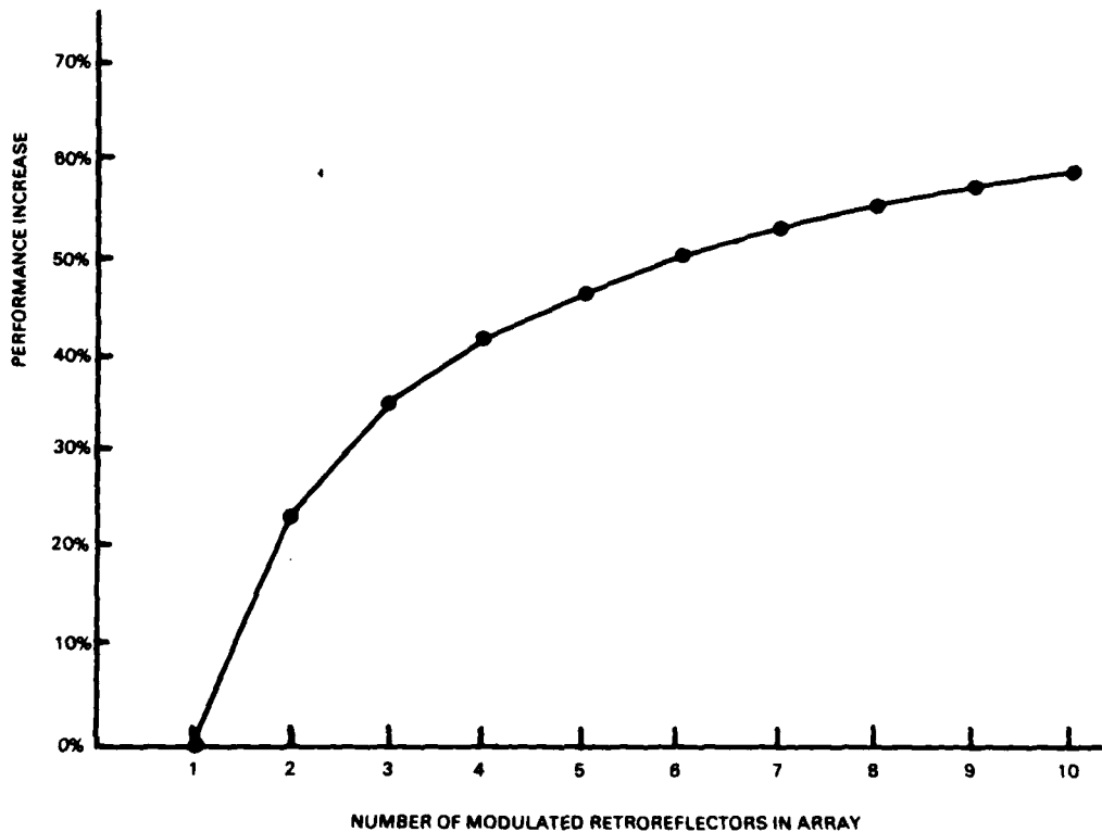
Figure 25. Performance increase in scintillation index reduction as a function of the number of modulated retroreflectors comprising the array for 8-cm separation using 0.633- \mu m light.
