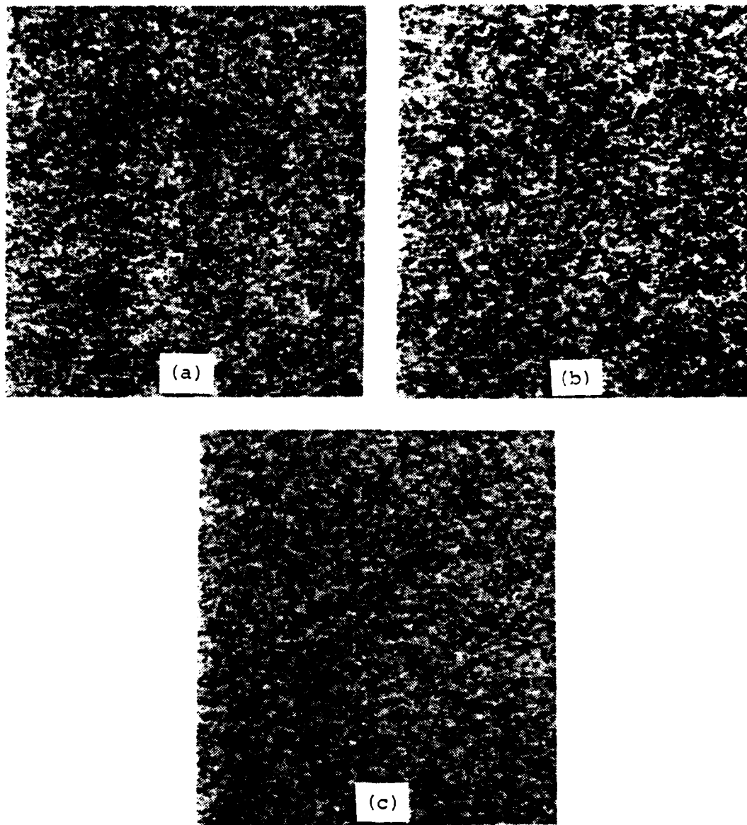
Figure 9. Optical micrographs of the HT-4 material after 850°C austenitization and subsequent isothermal transformation heat treatment at 275°C. After: (a) 10 seconds, (b) 5 minutes, and (c) 50 minutes. Micrographs indicated a slight coarsening of the grains. The grain size here is 3-4 μm. Etched in 5% nital solution. 250X.
