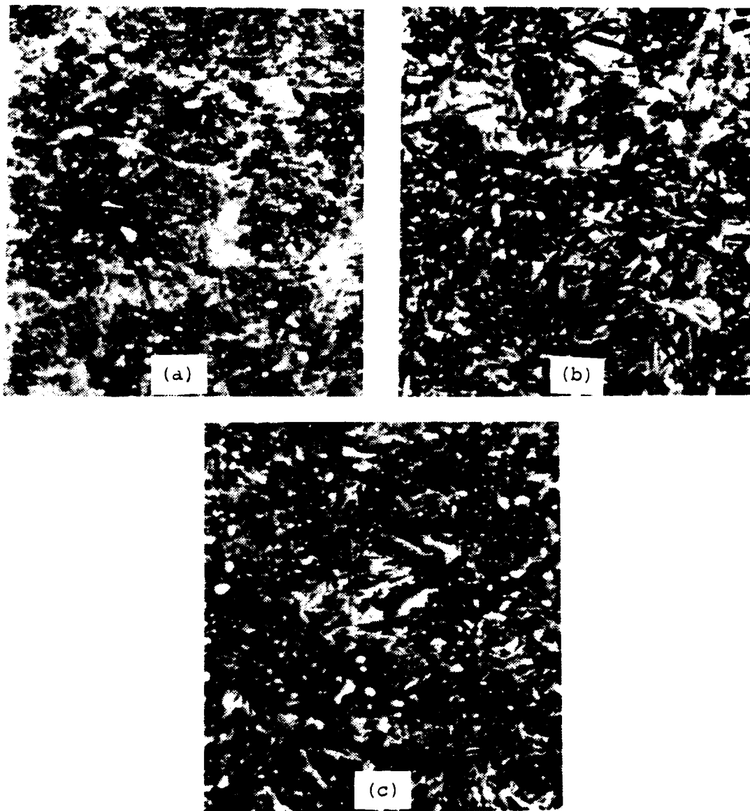
Figure 10. Optical micrographs of the AR material after 850°C austenitization and subsequent isothermal transformation heat treatment at 275°C. After (a) 5 seconds, (b) 10 minutes, and (c) 50 minutes. Also the microstructures are (a) martensite, (b) duplex martensite and bainite, and (c) bainite. Residual carbides are evident throughout. Etched in 5% nital. 1600X.
