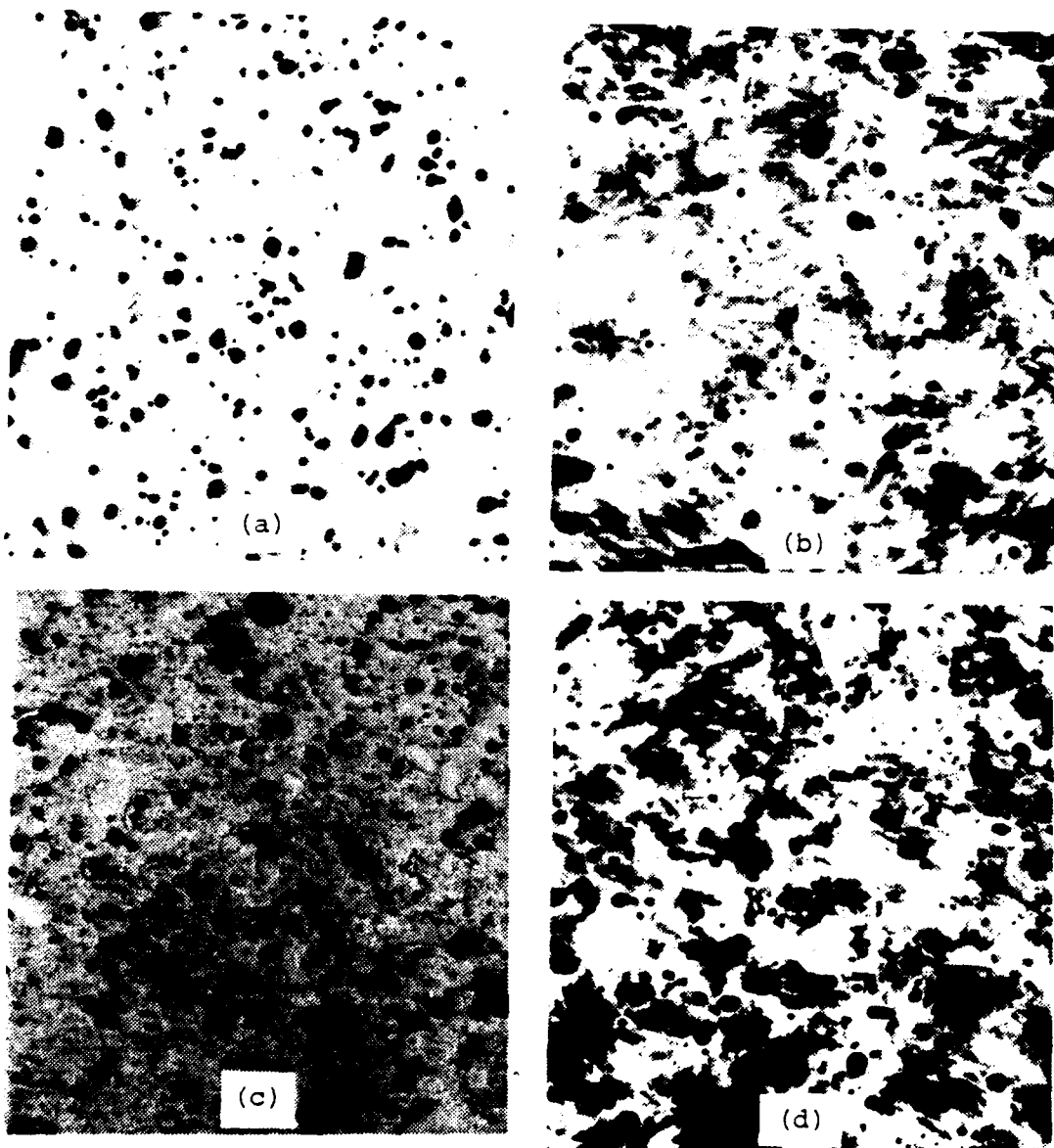
Figure 12. Carbide extraction replica micrographs of both the AR and HT-4 materials after 850°C austenitization and subsequent isothermal transformation heat treatment at 275°C. (a) AR after 5 seconds, (b) AR after 50 minutes, (c) HT-4 after 10 seconds, and (d) HT-4 after 50 minutes. The micrographs show the coarsening of the carbides after austenitization of the HT-4 material. 5000X.
