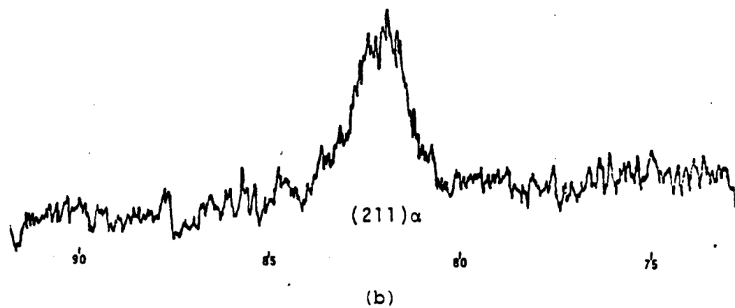
Figure 19. Autographic record of x-ray diffraction peaks for AR and HT-4 materials heat treated at 275°C. (a) Material AR after 5 seconds isothermal transformation. (b) Material HT-4 after 10 seconds of isothermal transformation. No retained austenite is evident.
