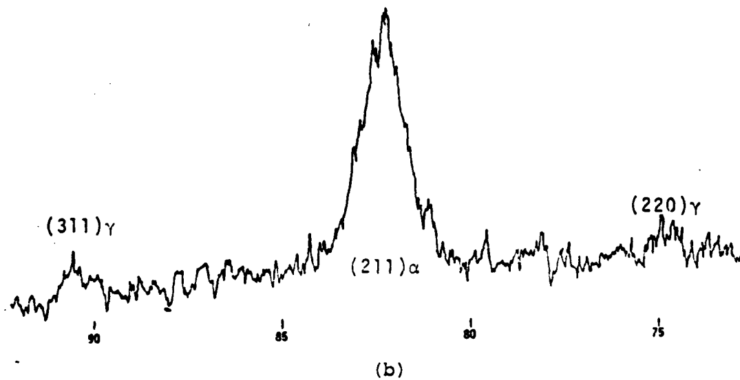
Figure 20. Autographic record of x-ray diffraction peaks for AR material heat treated at 250°C. (a) After 50 minutes of isothermal transformation, no retained austenite evident. (b) After 20 seconds of isothermal transformation, 6% retained austenite.
