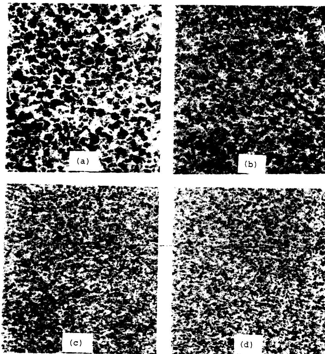
Figure 15. Optical micrographs of both the AR and HT-4 materials after 850^{\circ}\text{C} austenitization and subsequent isothermal transformation heat treatment at 250^{\circ}\text{C} . (a) AR after 20 seconds, (b) AR after 50 minutes, (c) HT-4 after 10 seconds, and (d) HT-4 after 50 minutes. The microstructure in (a & c) is martensite, in (b) is bainite and in (d) is a duplex martensite and bainite. Etched in 5% nital solution. 250X.
