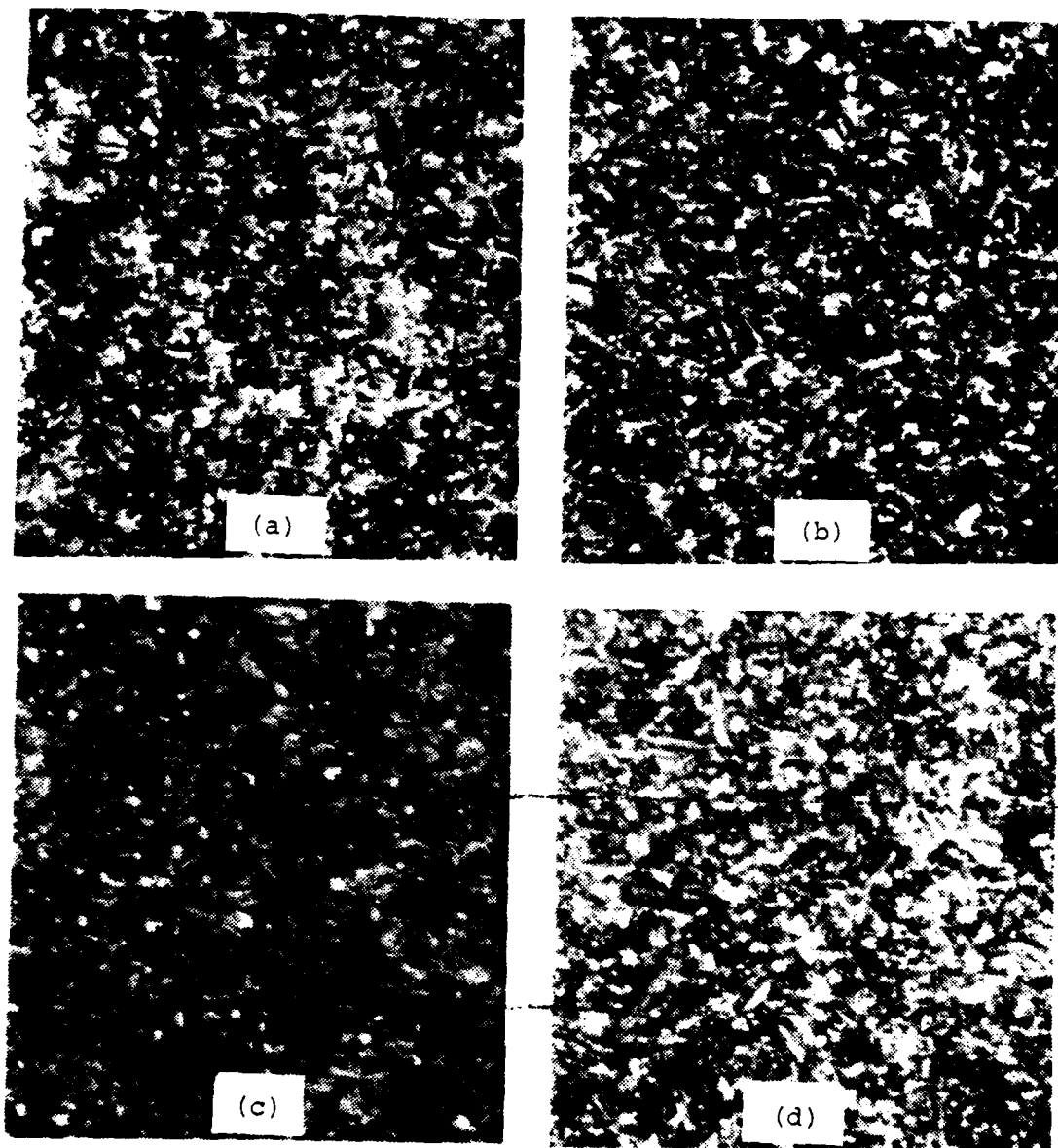
Figure 16. Optical micrographs of both the AR and HT-4 materials after 850°C austenitization and subsequent isothermal transformation heat treatment at 250°C. (a) AR after 20 seconds, (b) AR after 50 minutes, (c) HT-4 after 10 seconds, and (d) HT-4 after 50 minutes. Microstructures are residual carbides and martensite in (a & c), bainite in (b), and (d) is a duplex martensite and bainite. Etched in 5% nital solution. 1600X.
