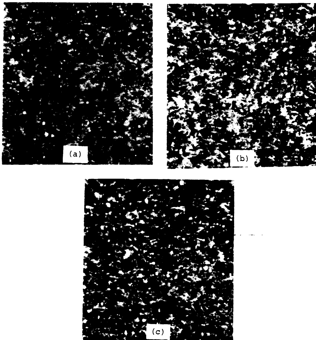
Figure 11. Optical micrographs of the HT-4 material after 850°C austenitization and subsequent isothermal transformation heat treatment at 275°C. After (a) 10 seconds, (b) 5 minutes, and (c) 50 minutes. The microstructures are: (a) martensite, (b) duplex martensite and bainite, and (c) bainite. The carbides coarsened during austenitization are evident. Etched in 5% nital solution. 1600X.
