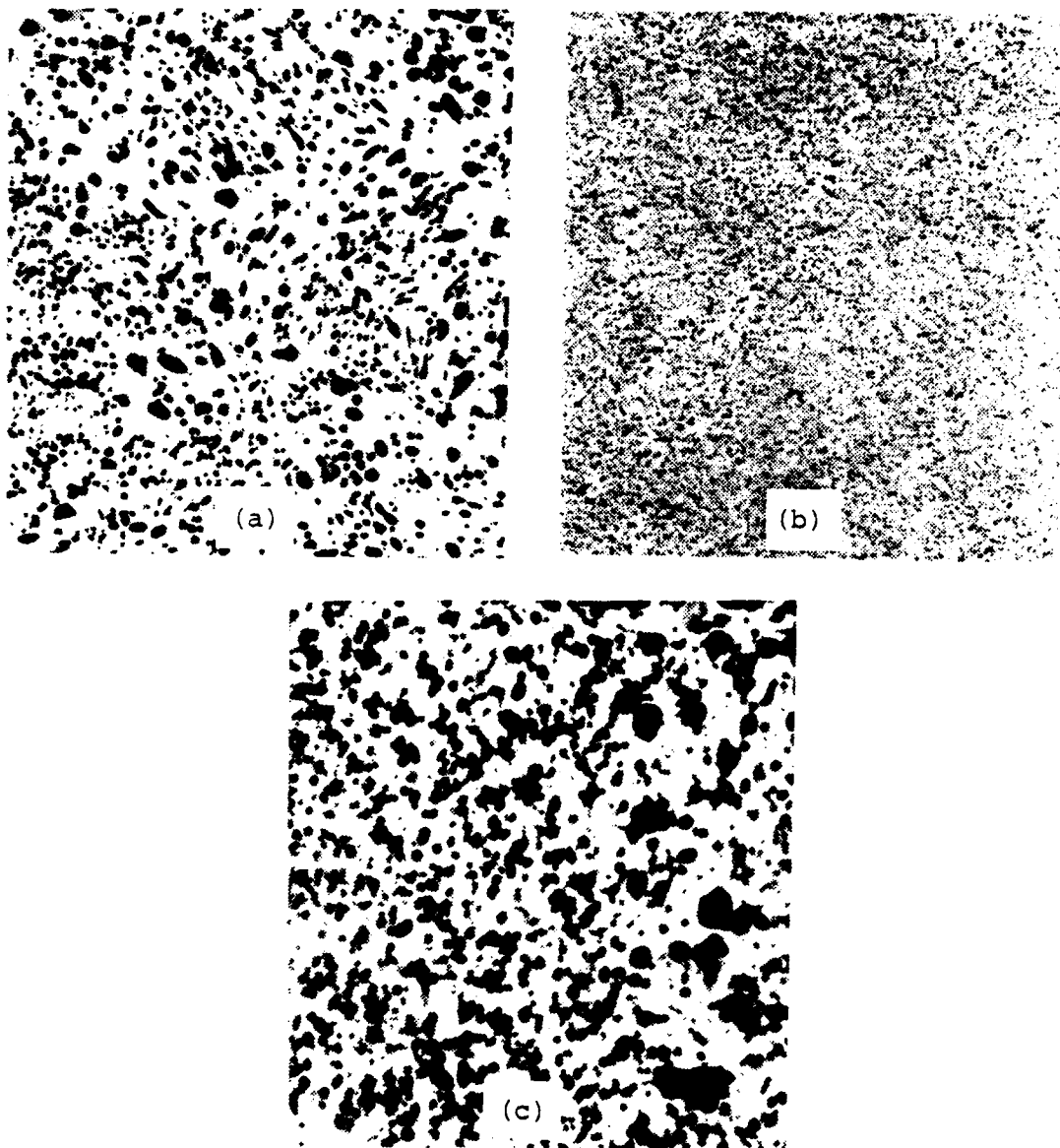
Figure 4. Carbide extraction transmission electron micrographs of AISI 52100 steel. (a) standard spheroidize annealed carbide microstructure, (b) thermomechanically refined HT-4 carbide microstructure consisting of submicron residual and tempered carbides. 1400X. (c) carbide extraction micrograph of overly extracted thermomechanically refined HT-4 material. 5000X.
