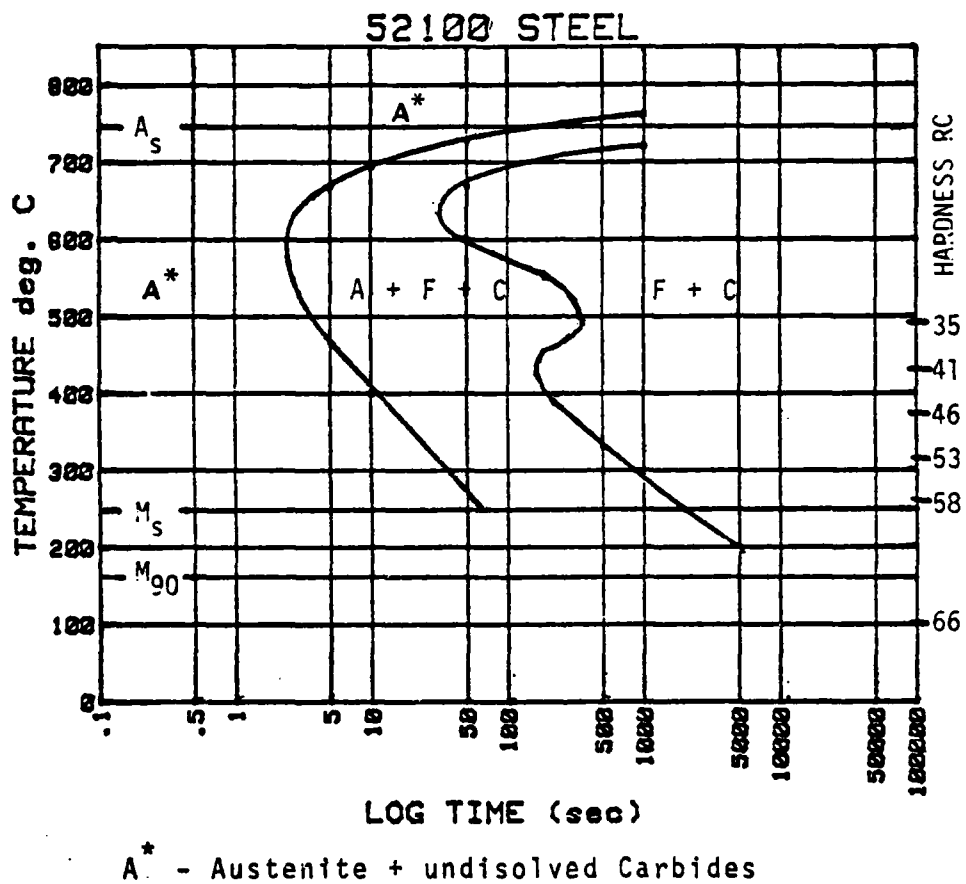
Figure 1. Isothermal transformation diagram for 52100 steel. Applicable for austenitizing at 850°C and for an ASTM grain size of 9. Adapted from Reference 11.
