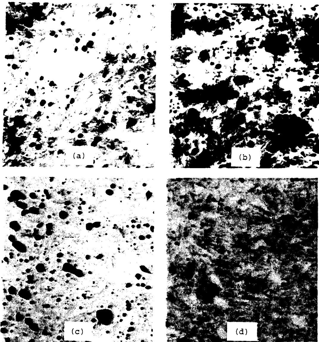
Figure 18. Carbide extraction replica micrographs of both the AR and HT-4 materials after 850°C austenitization and subsequent isothermal transformation heat treatment at 250°C. (a) AR after 10 minutes is duplex martensite and bainite, (b) AR after 50 minutes is bainite, (c) HT-4 after 10 seconds is martensite, and (d) HT-4 after 50 minutes is martensite. Residual carbides are evident throughout. 5000X.
