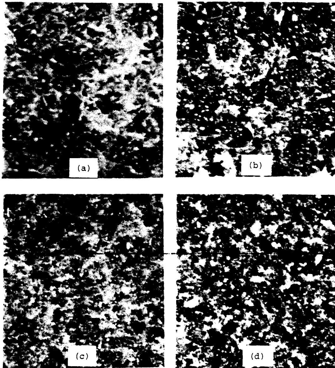
Figure 14. Optical micrographs of both the AR and HT-4 materials after 850°C austenitization and subsequent isothermal transformation heat treatment at 350°C. (a) AR after 20 seconds, (b) AR after 20 minutes, (c) HT-4 after 10 seconds, and (d) HT-4 after 20 minutes. Microstructures are (a & c) martensite and residual carbides and (b & d) bainite and residual carbides. Etched in 5% nital solution. 1600X.
