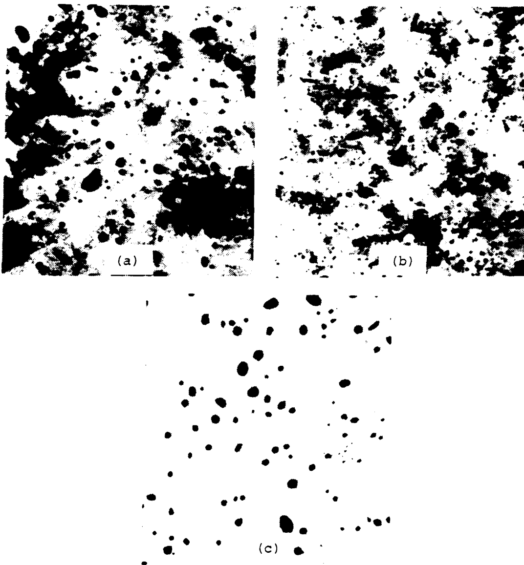
Figure 17. Carbide extraction replica micrographs of both the AR and HT-4 materials after 850°C austenitization and subsequent isothermal transformation heat treatment at 350°C. (a) HT-4 after 90 seconds, (b) HT-4 after 50 minutes, and (c) AR after 20 seconds. Microstructures show the coarsening of HT-4 carbides after austenitization and the dark feathery bainite. The AR microstructure is martensite with residual carbides. 5000X.
