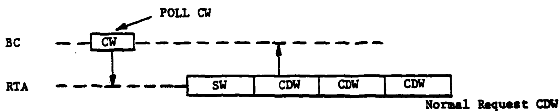
(a) Basic Poll/Request Sequence
