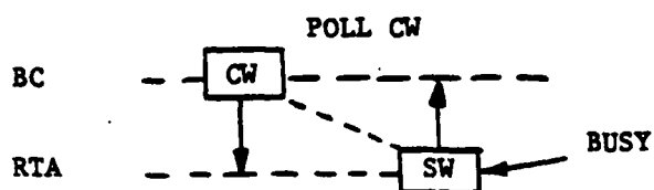
(b) Poll with Busy
