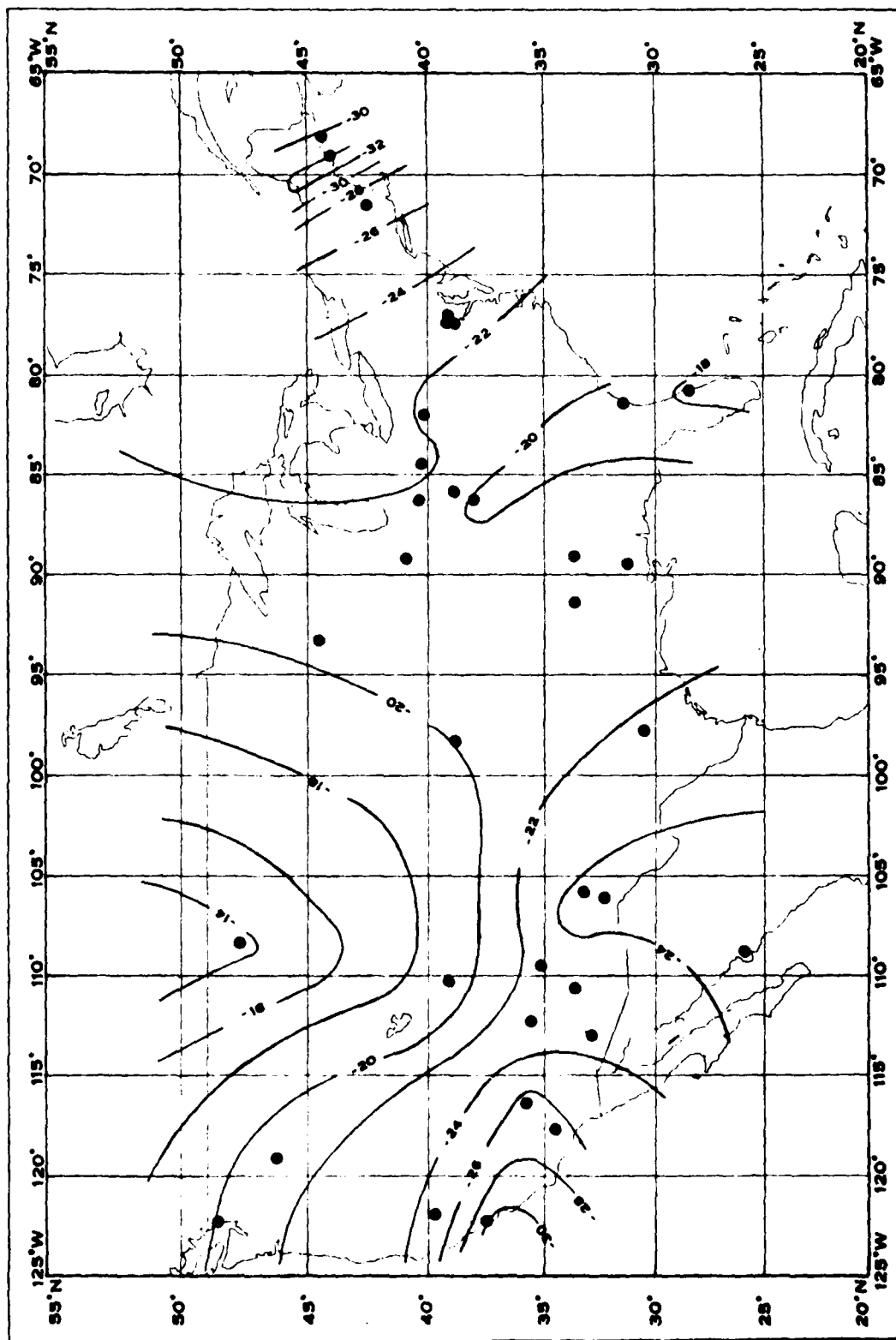
Figure 6. Contour Chart - NAD 27 to WGS 72 Datum Shifts, ΔX Component (Contour Interval = 2 meters).
