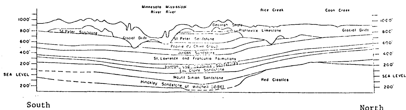
Figure 20. North-South Vertical Section Through the West End of Pike Island Showing the Twin Cities Artesian Basin (From Winter and Norvitch, 1972)
