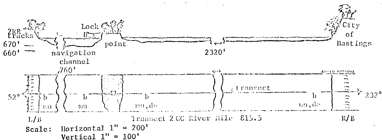
Figure 47. Schematic Diagrams of Riverscape Profiles, Plant and Animal Sampling Locations, and Bottom Types at Each Standard Transect in Pool 2 (Cudmundson, 1973).
