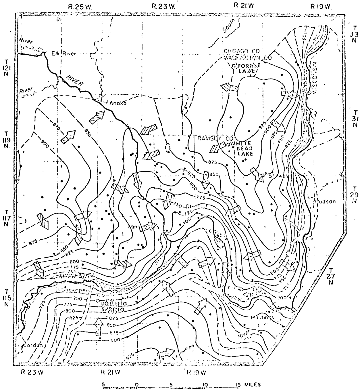
Figure 26. Potentiometric Surface of Water in the Prairie du Chien-Jordan Aquifer in Winter 1970-71, in the Minneapolis-St. Paul Area (Winter and Norvitch, 1972)
