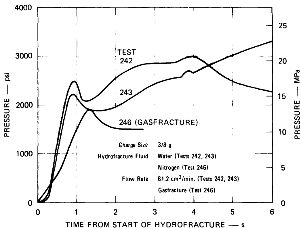
FIGURE 3.14 GASFRACTURE AND HYDROFRACTURE PRESSURES FOR VENTED EXPLODED CAVITY TESTS 242, 243, AND 246
