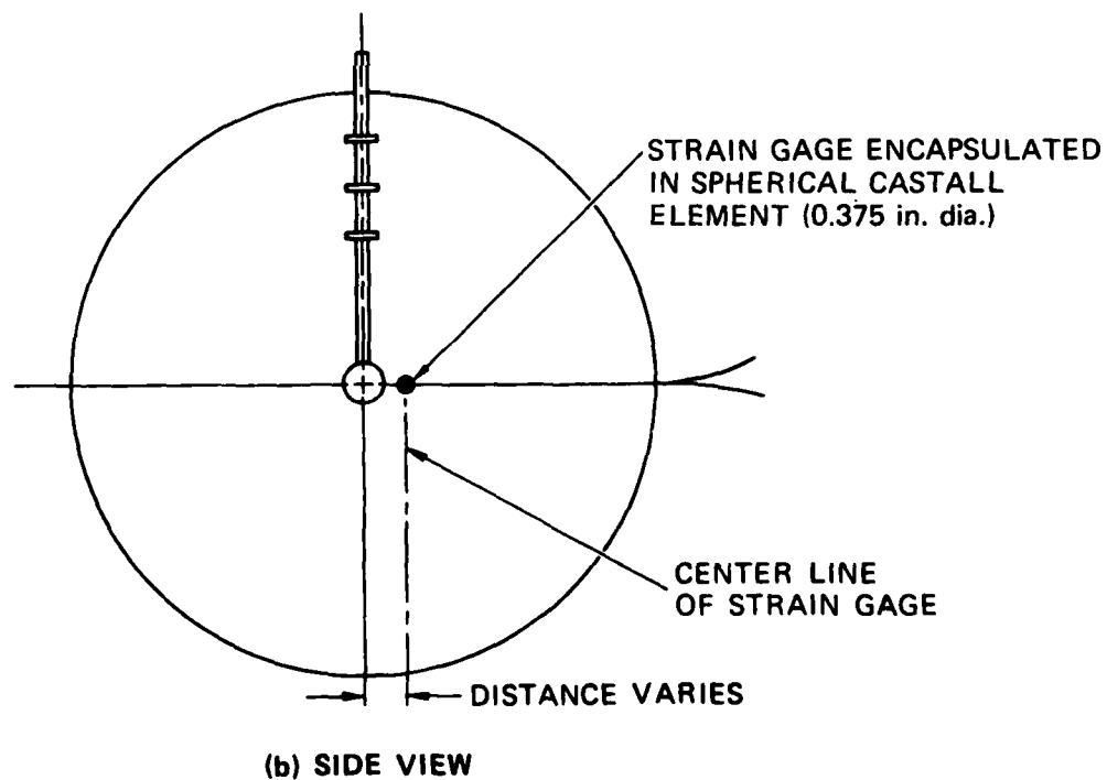
FIGURE 2.11 EMBEDDED STRAIN GAGE
