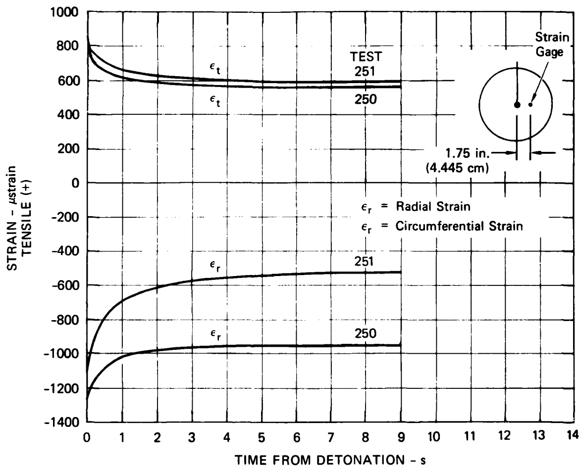
FIGURE 3.15 RESIDUAL RADIAL AND CIRCUMFERENTIAL STRAIN FOR UNVENTED EXPLODED CAVITY TESTS 250 AND 251
