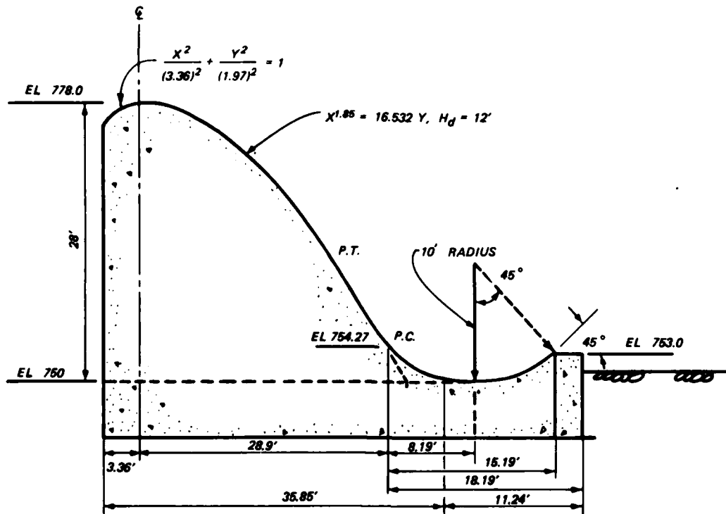
Figure 6. Type 4 design energy dissipator
