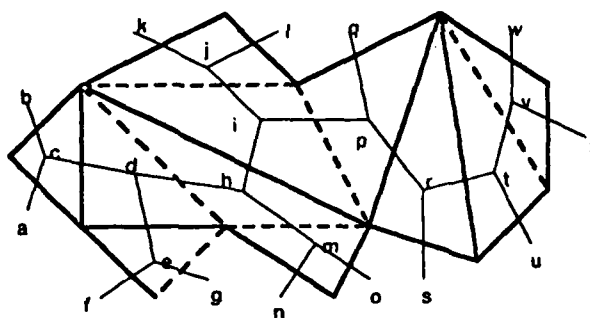
Figure 2.4 Taking the dual of \text{TRI}(G) to form T
