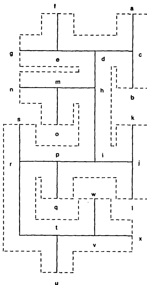
Figure 2.5 T and the regions between adjacent leaves
