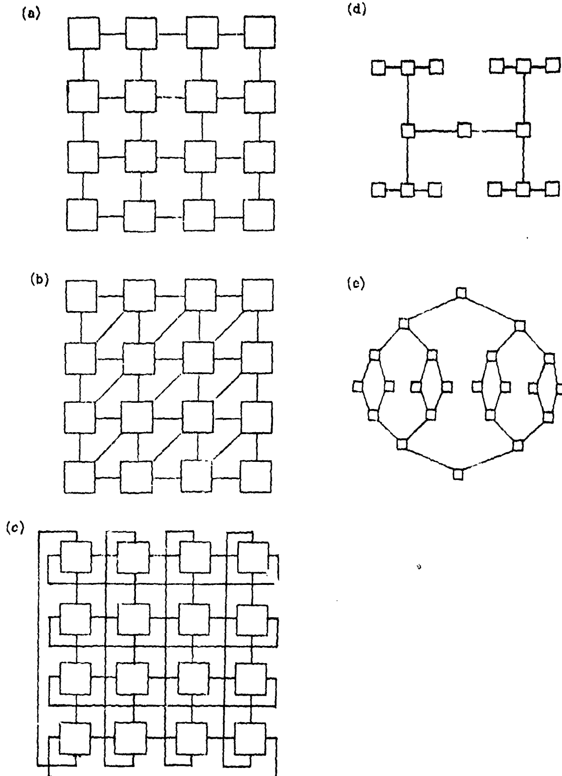
Figure 1. Interconnection patterns for parallel algorithms (a) mesh, (b) hexagonally connected mesh, (c) torus, (d) binary tree, (e) double tree.
